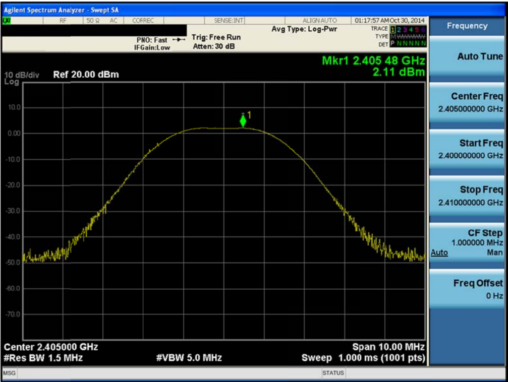
Maximum Peak Conducted Output Power TM1 & Lowest channel
