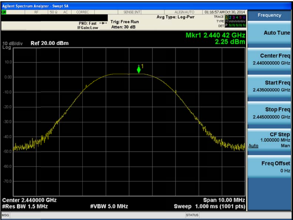
Maximum Peak Conducted Output Power TM1 & Middle channel
