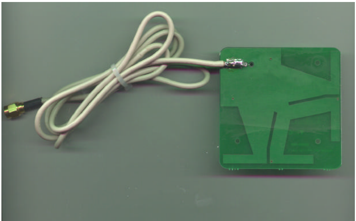
Figure 24: ISA Antenna Inside (Front)
