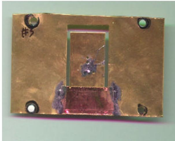
Bottom Solder Side Antenna (6dBi)
