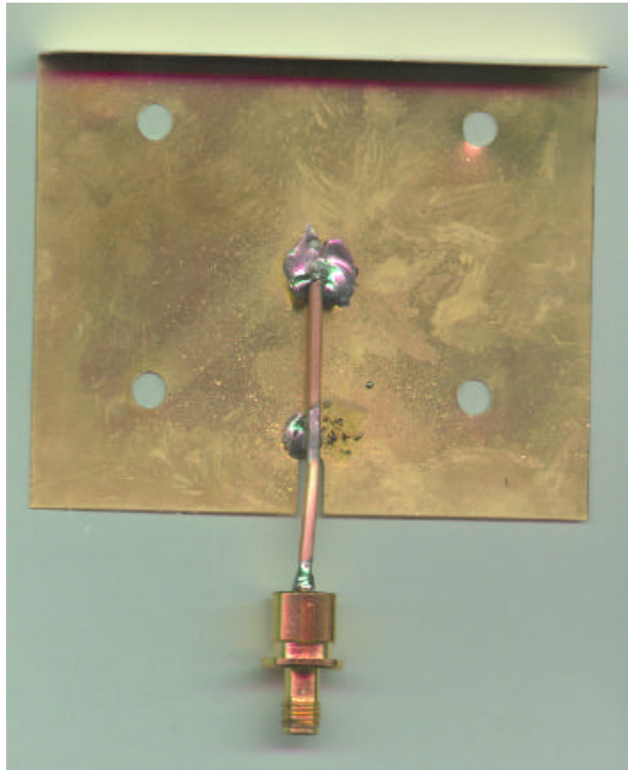
Top Solder Antenna (6dBi)
