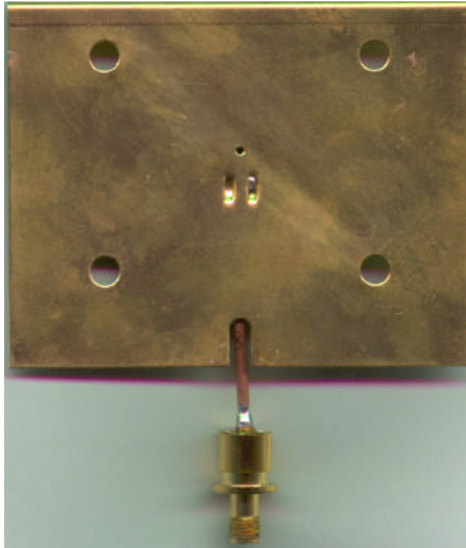
Top Component Antenna (6dBi)
