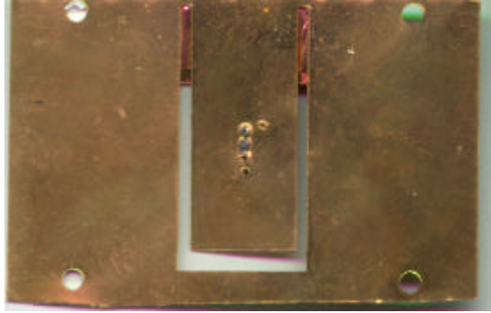
Bottom Component Side Antenna (6dBi)
