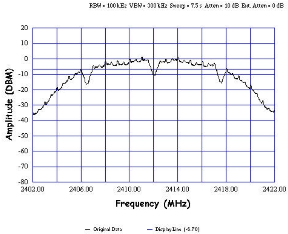
FIGURE 3: 6dB Occupied Bandwidth (Channel 1)
