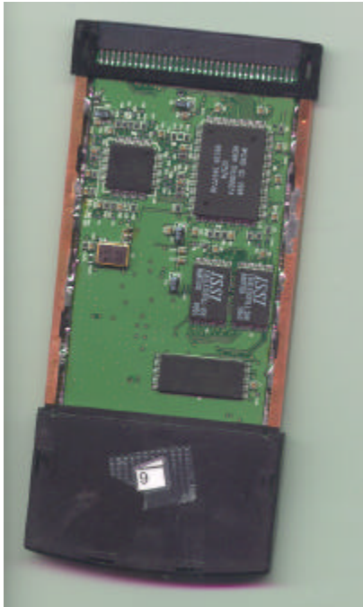
Figure 23: PCM Solder Side
