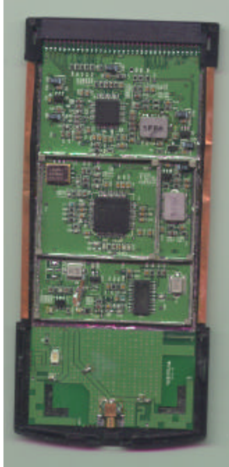
Figure 22: PCM Component Side
