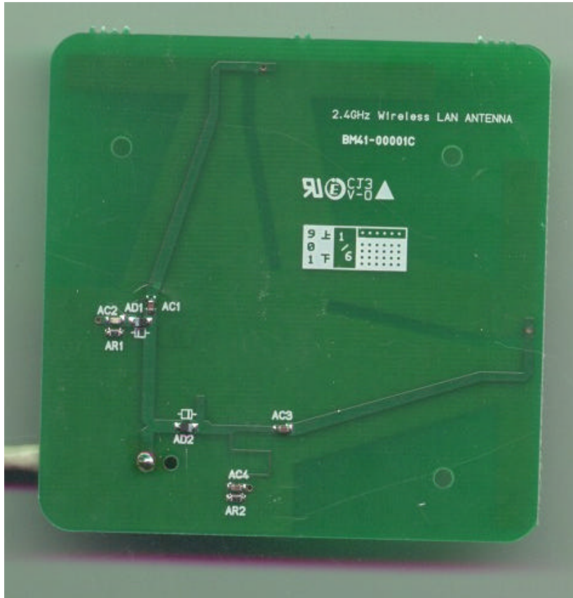
Figure 25: Patch Antenna Component Side
