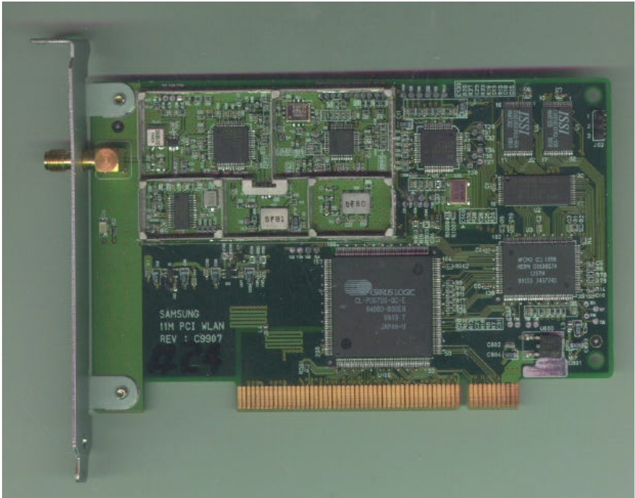
Figure 22: PCI Board Component Side
