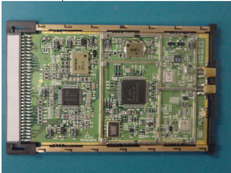
Top view of the board without the main cover
