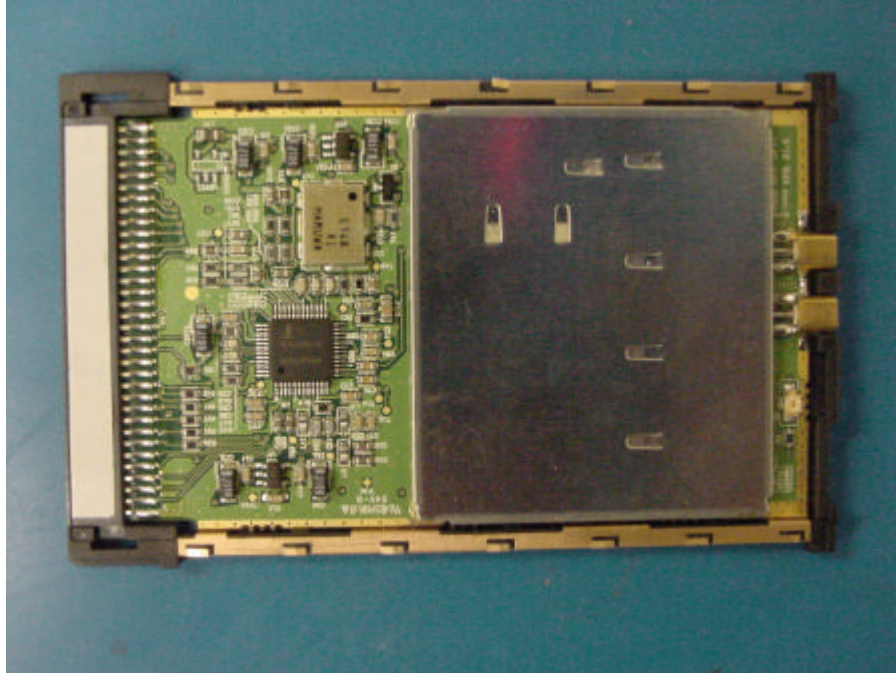
Top view of the board
