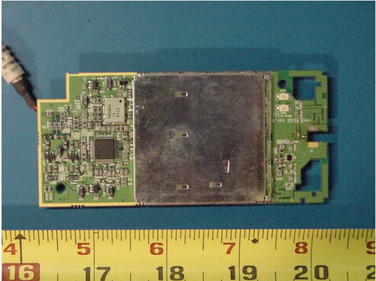
PHOTOGRAPH 10: BOTTOM VIEW OF THE BOARD WITH CAN
