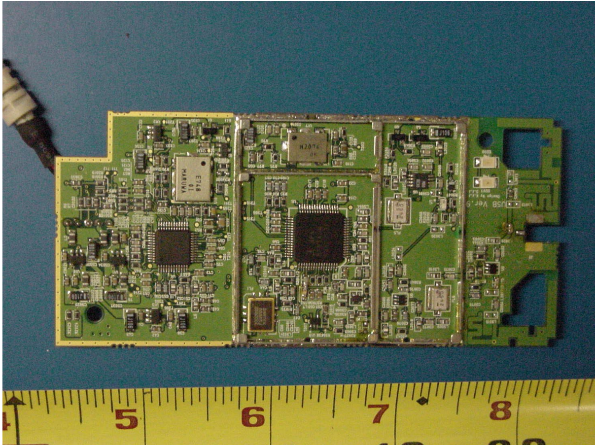
PHOTOGRAPH 9: BOTTOM VIEW OF THE BOARD WITHOUT CAN
