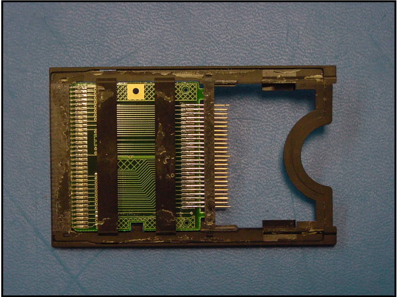
PHOTOGRAPH 16: REAR VIEW OF ADAPTER
