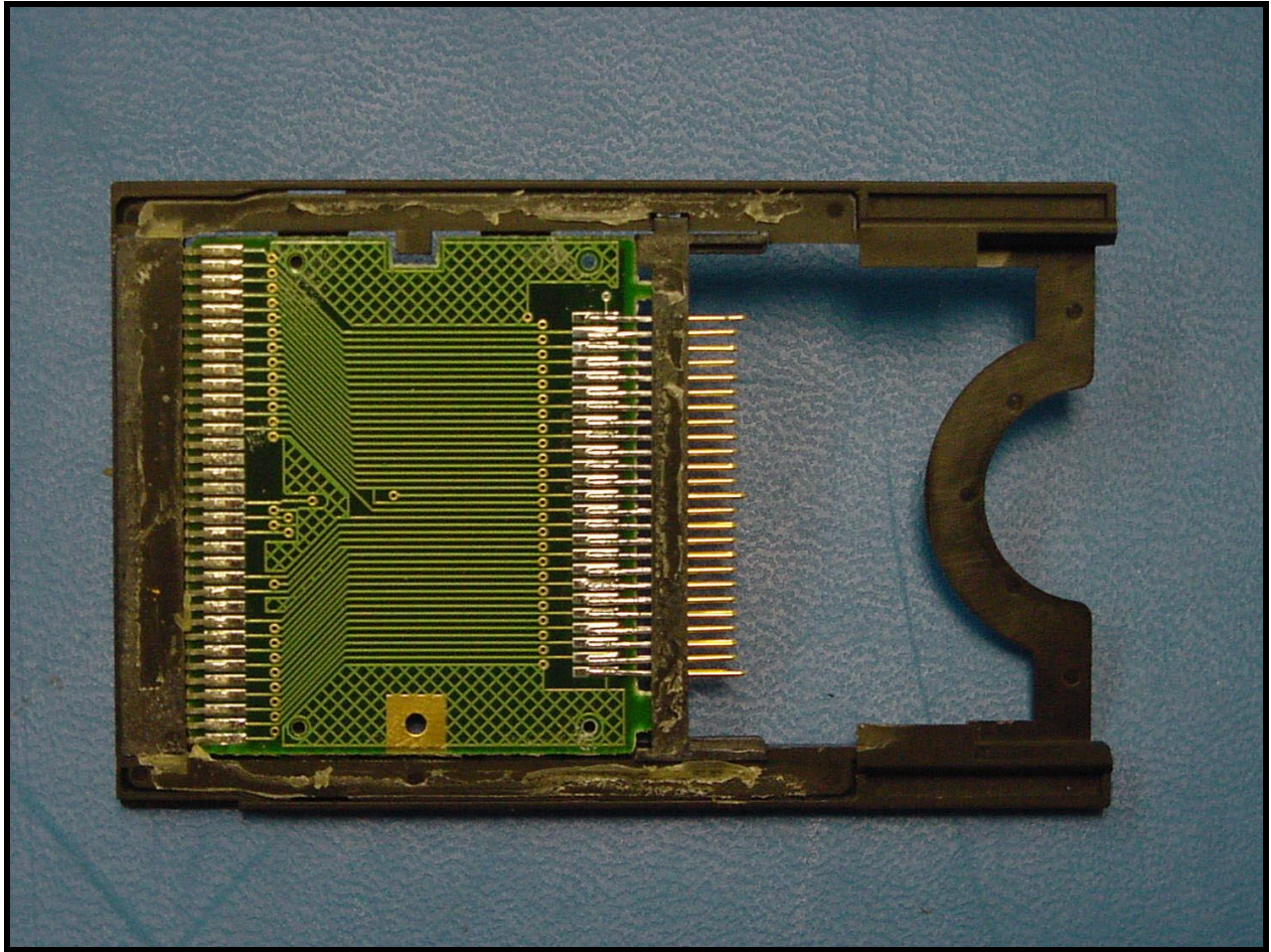
PHOTOGRAPH 15: FRONT VIEW OF ADAPTER
