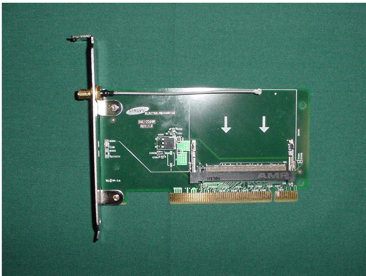
PHOTOGRAPH 12: FRONT OF PCI CARD WITHOUT MINI PCI WLAN RADIO
