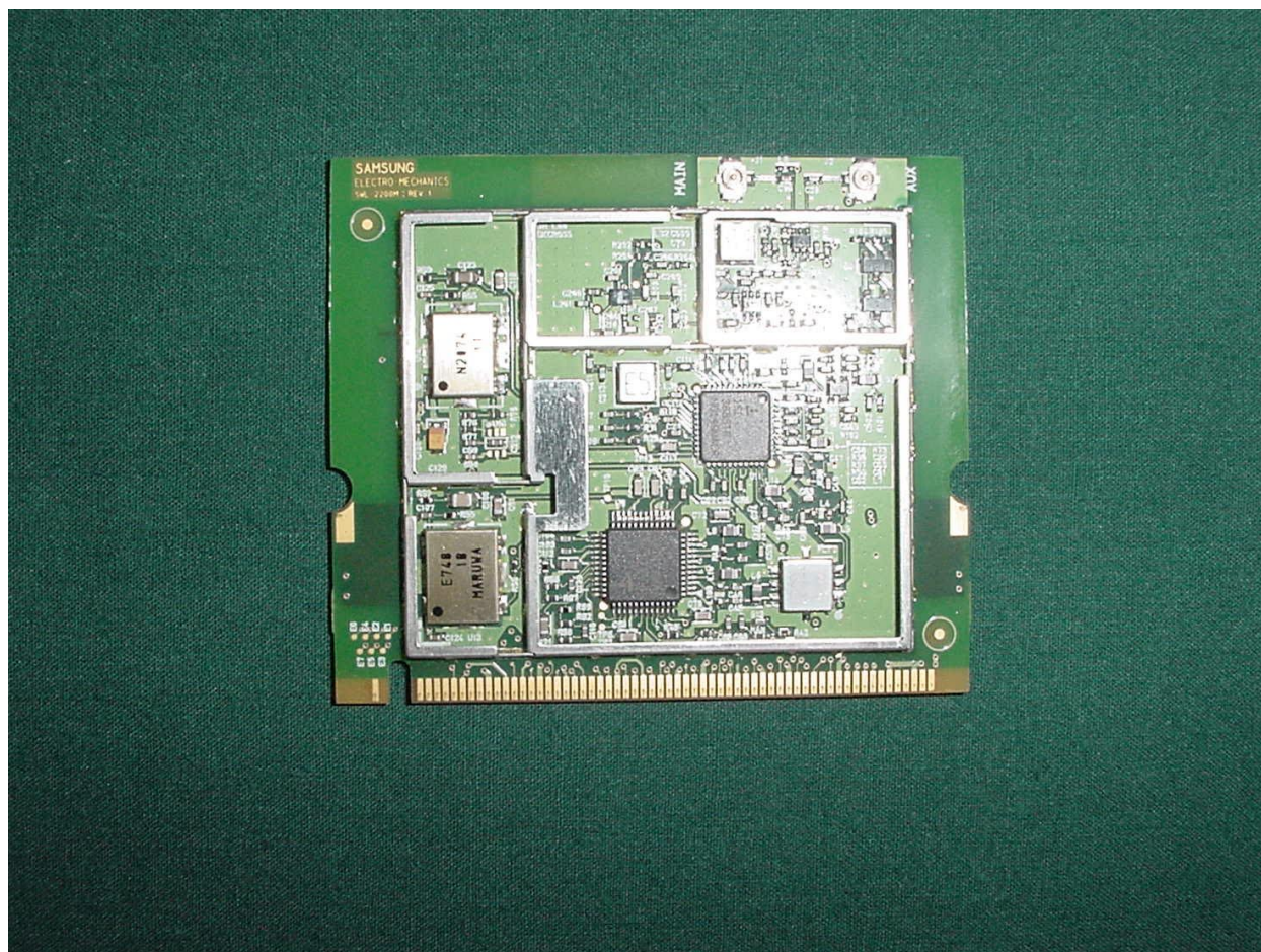
PHOTOGRAPH 15: FRONT VIEW OF 2200M WITHOUT SHIELD
