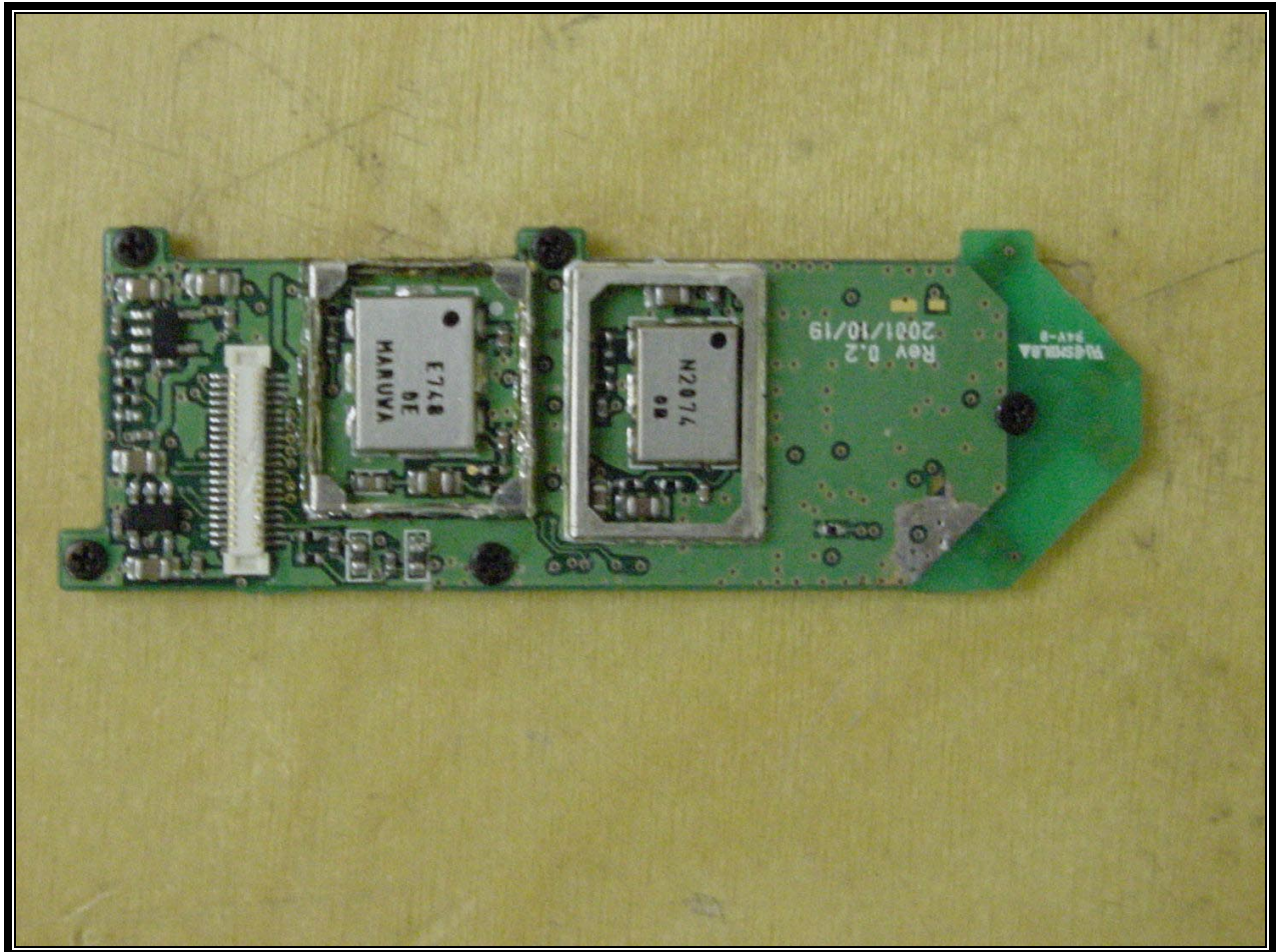
PHOTOGRAPH 11: BOTTOM VIEW OF RF BOARD WITHOUT SHIELD
