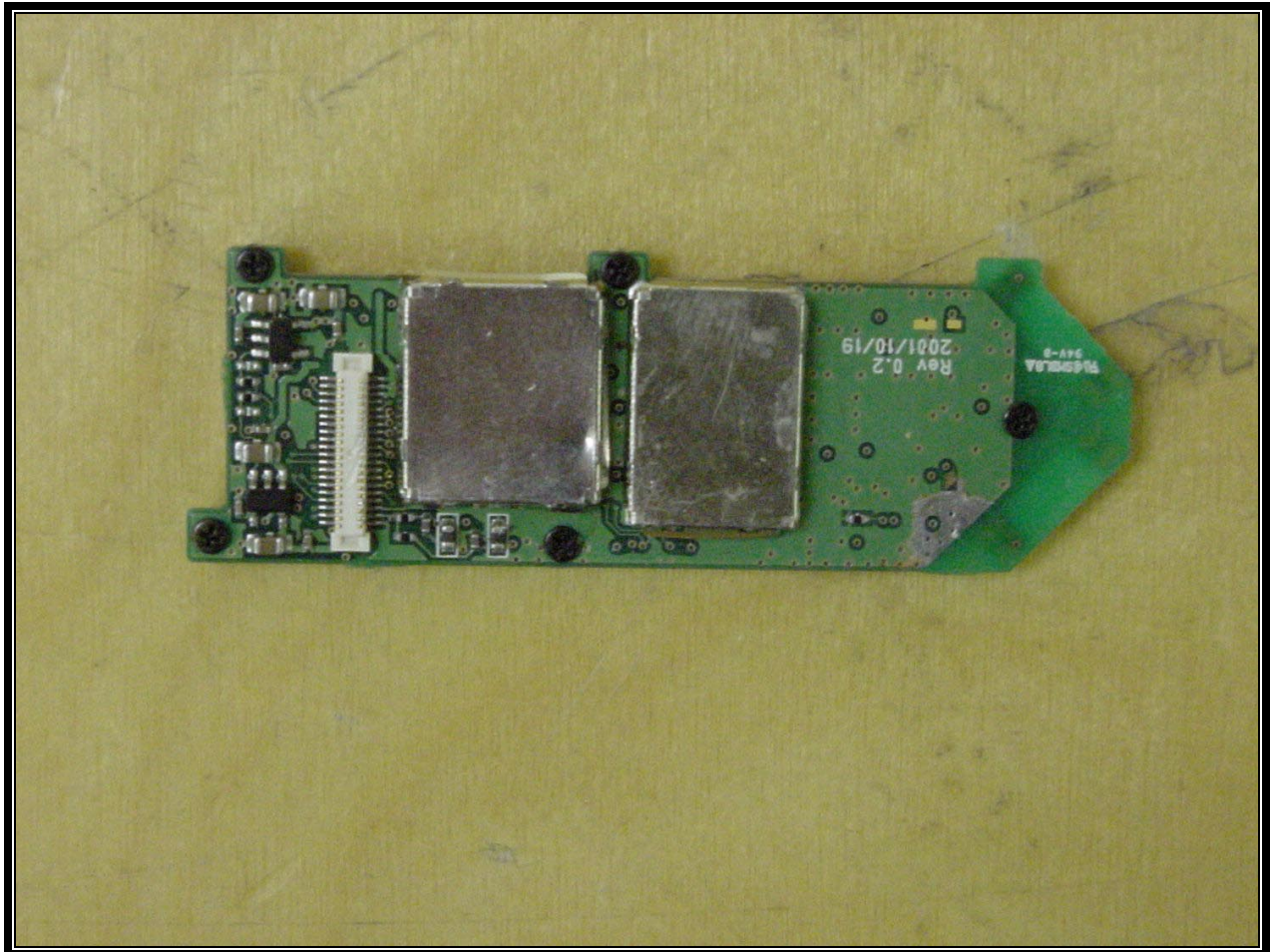
PHOTOGRAPH 10: BOTTOM VIEW OF RF BOARD WITH SHIELD
