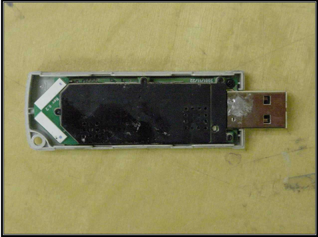
PHOTOGRAPH 9: TOP VIEW OF RF BOARD
