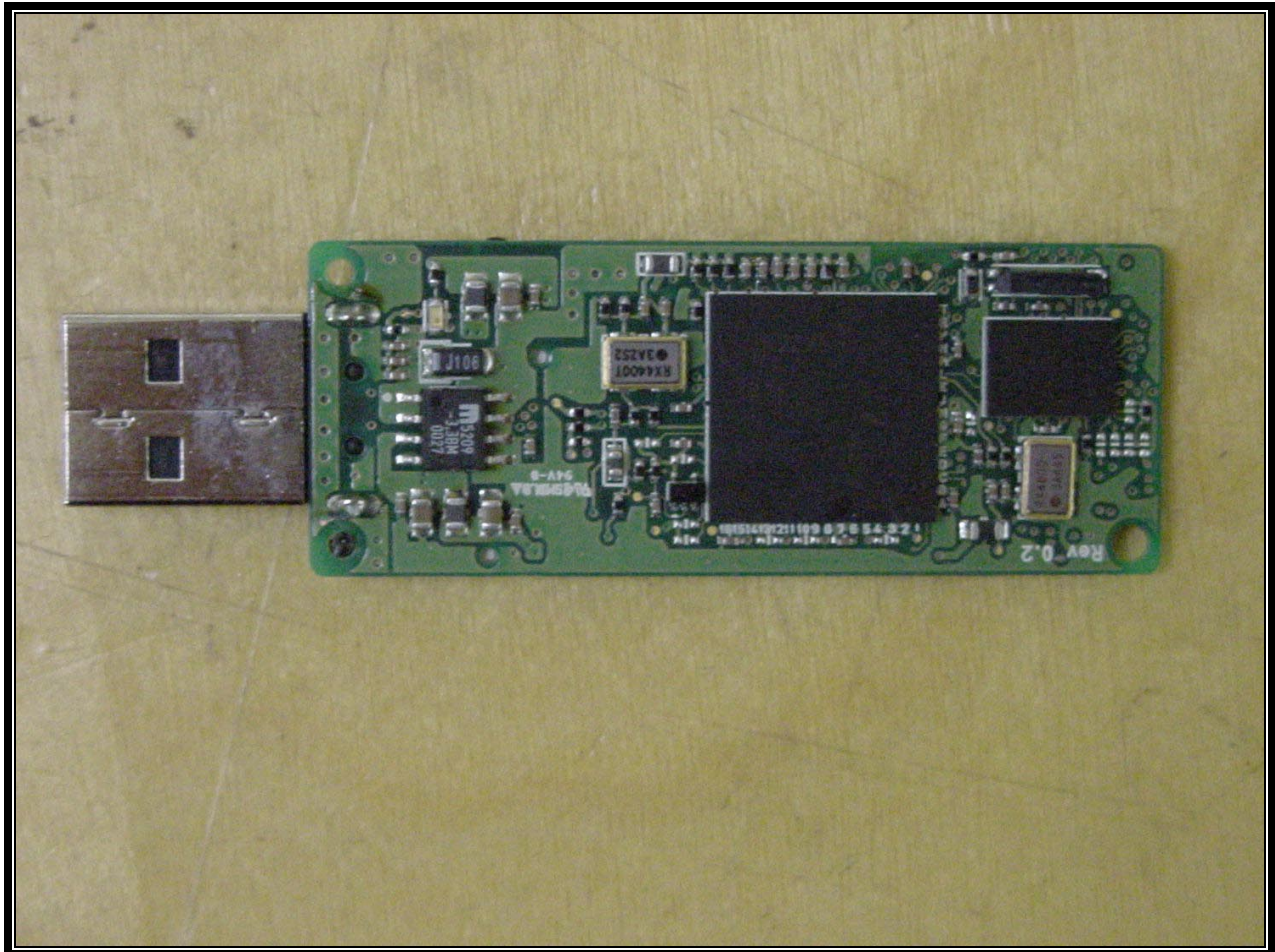
PHOTOGRAPH 13: BOTTOM VIEW OF DIGITAL BOARD
