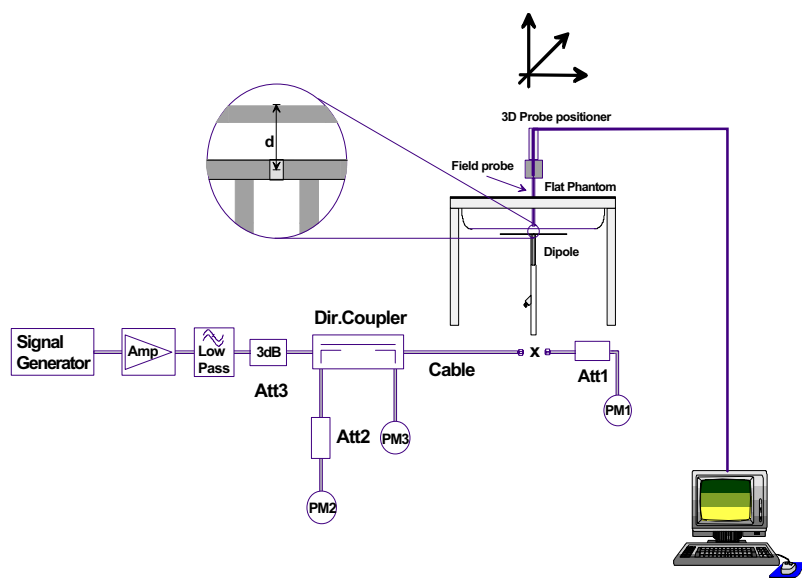
Figure 6. 2450MHz System Check Setup Diagram
