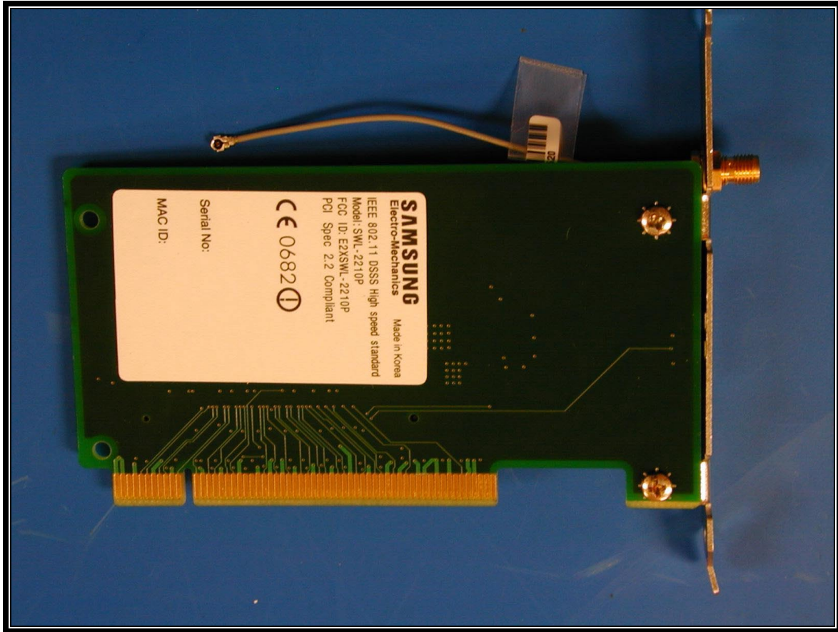
PHOTOGRAPH 8: BACK VIEW SWL-2210P
