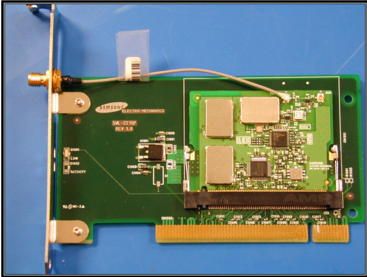
PHOTOGRAPH 7: FRONT VIEW SWL-2210P WITH SWL-2210M
