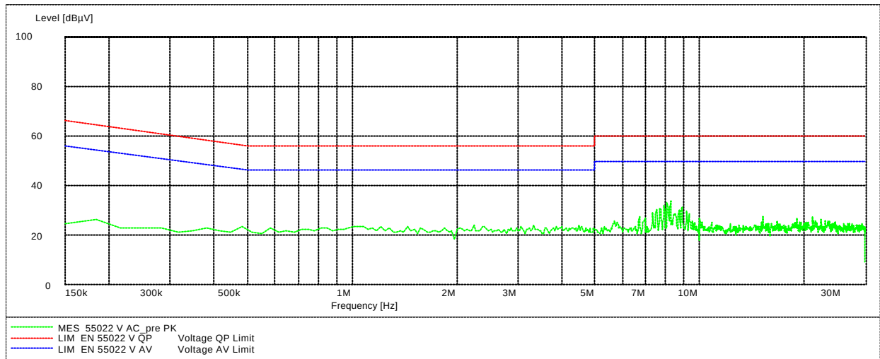
Plot 1: CISPR 22
