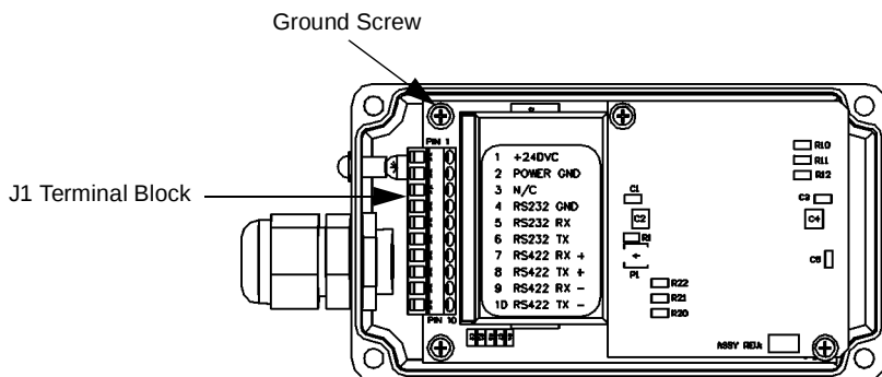
Figure 3-1. Internal junction block
