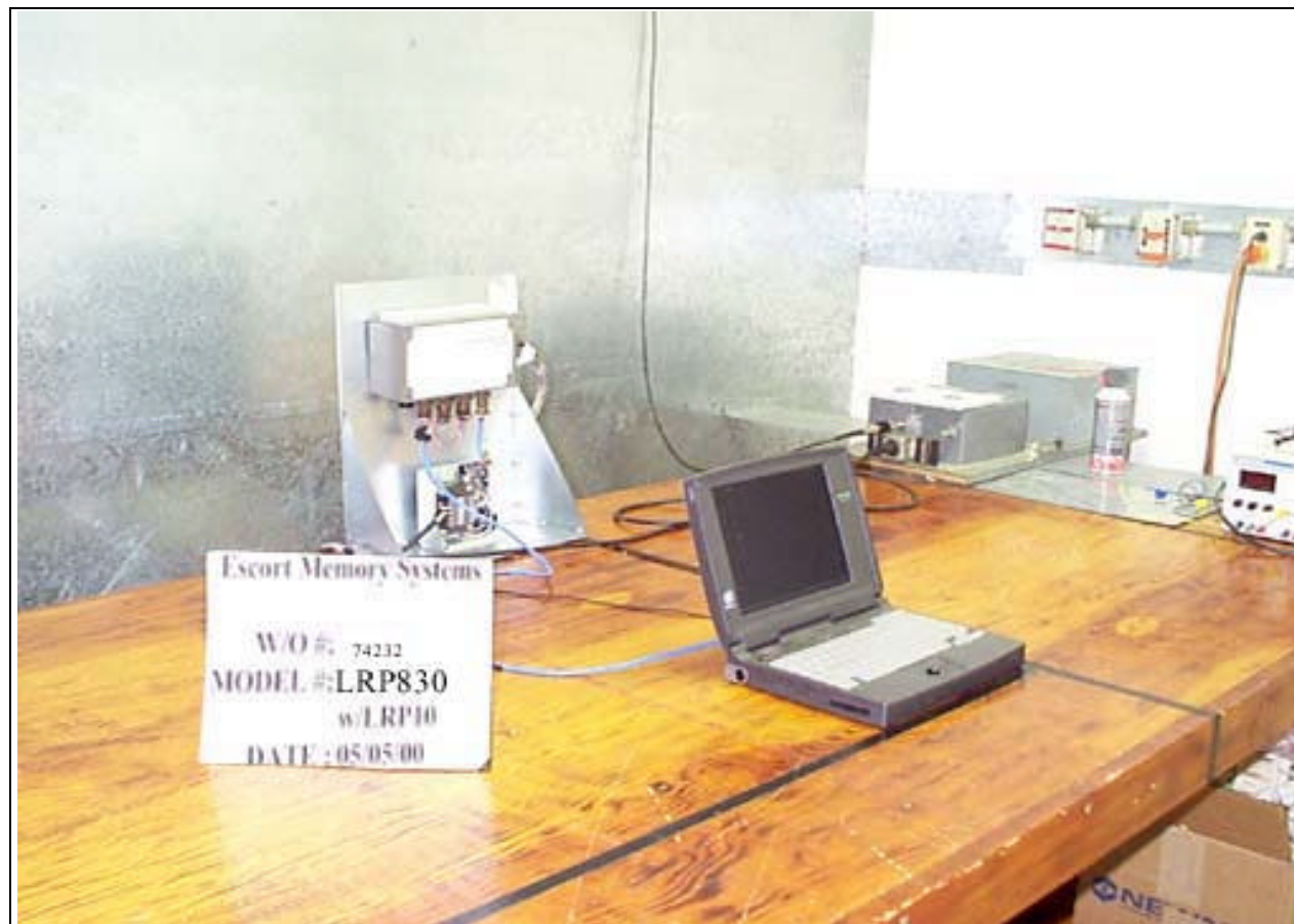
Conducted Emissions - Front View with DC Load
