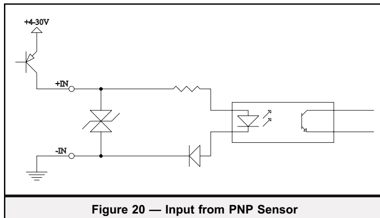
Figure 20 shows an Open Collector PNP output from a photosensor switches to the positive supply. It can be wired as a sourcing or high-side contact.
