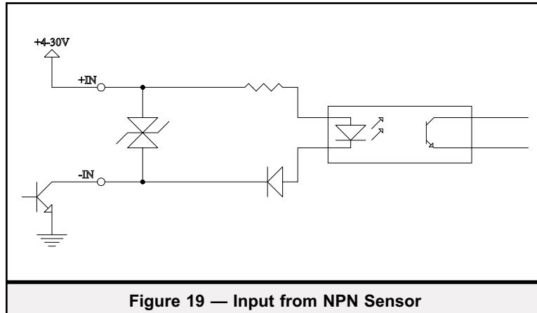
Figure 19 shows an Open Collector NPN output from a photosensor switching to ground. It can be wired as a sinking or low-side contact.
