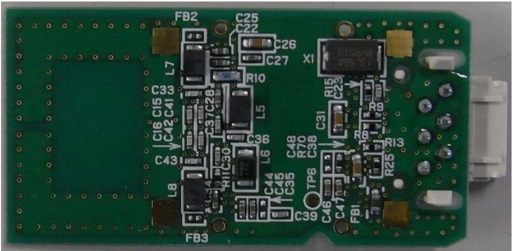
Rear
