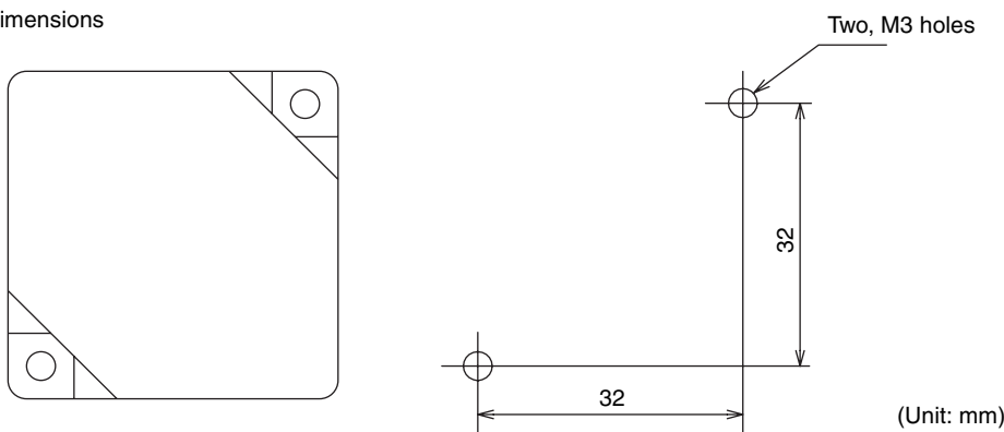
Mounting Hole Dimensions
