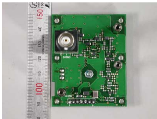
Side B (Reception circuit)
