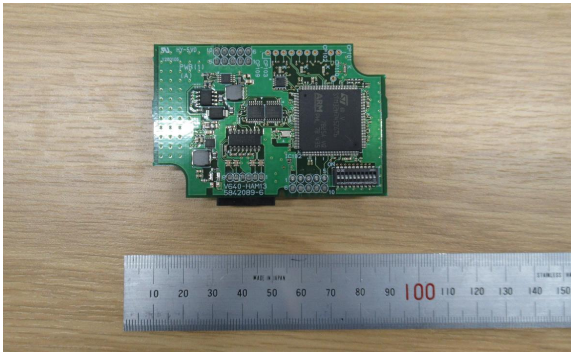
PCB(1) – Side A (74.4 x 49.4 mm)
