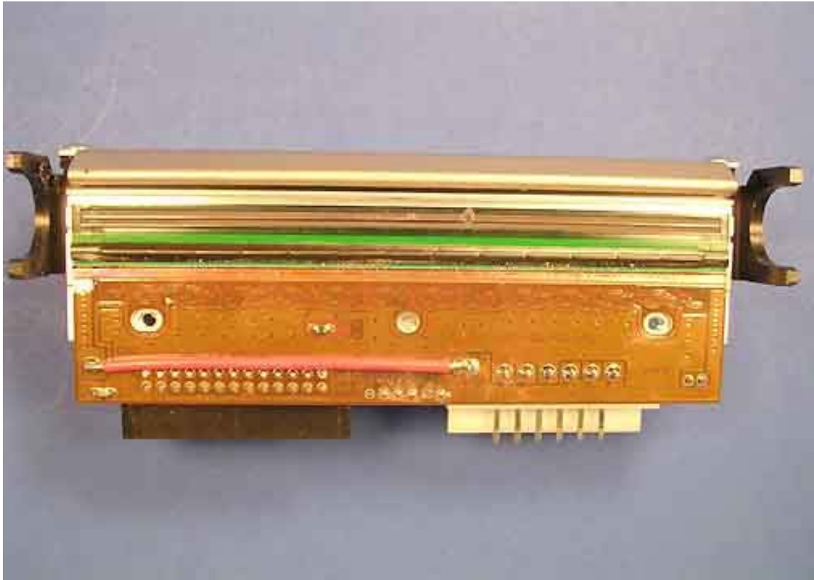
Board 1 Bottom
