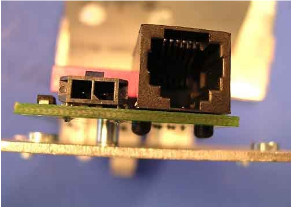
RFID Interface Board Front
