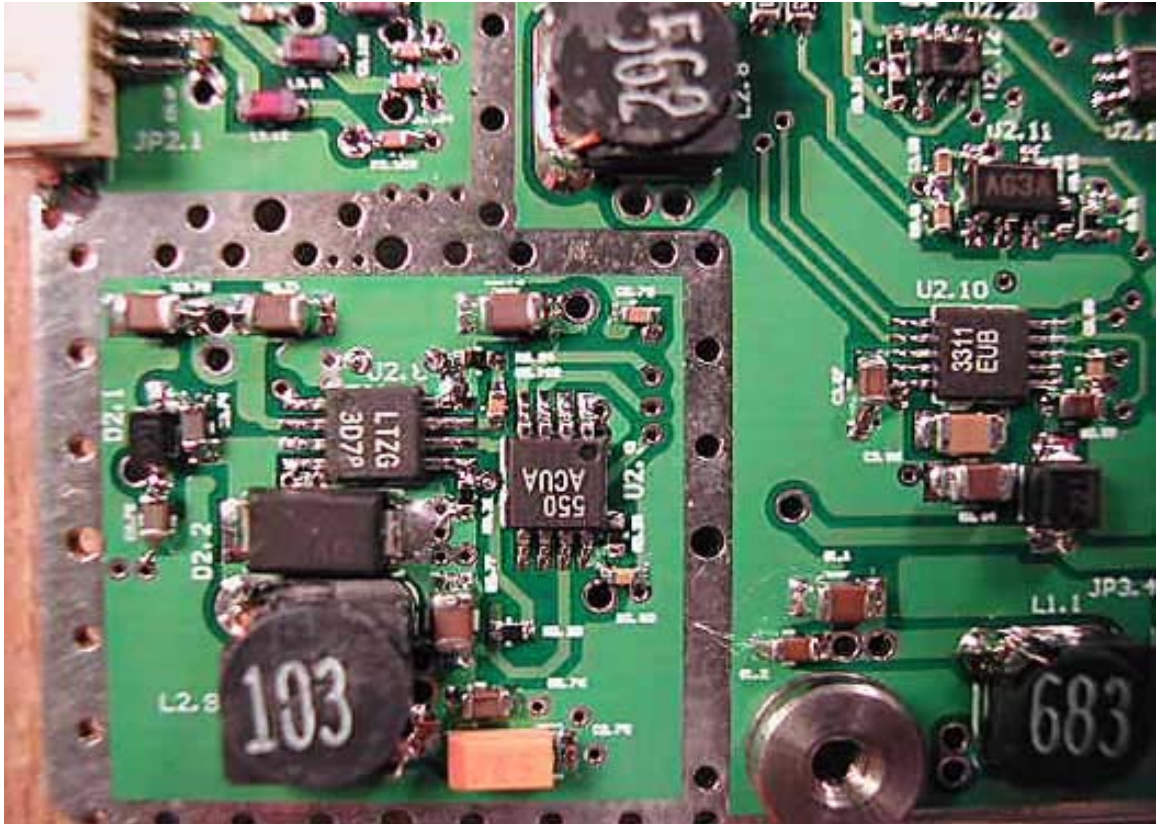
PCB Front 4
