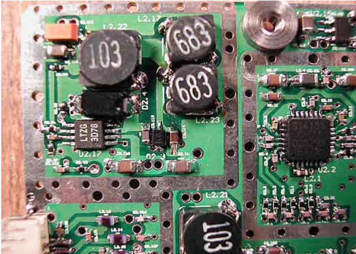
PCB Front 2
