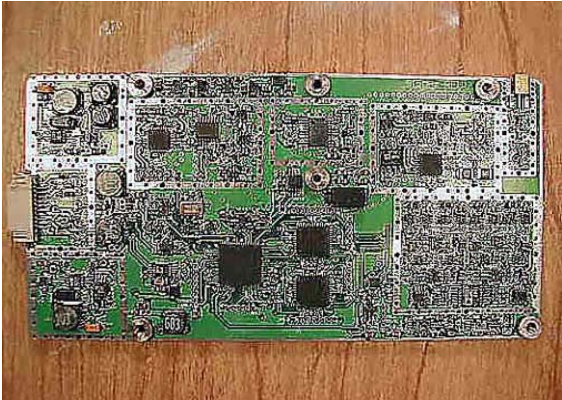
PCB Front 1
