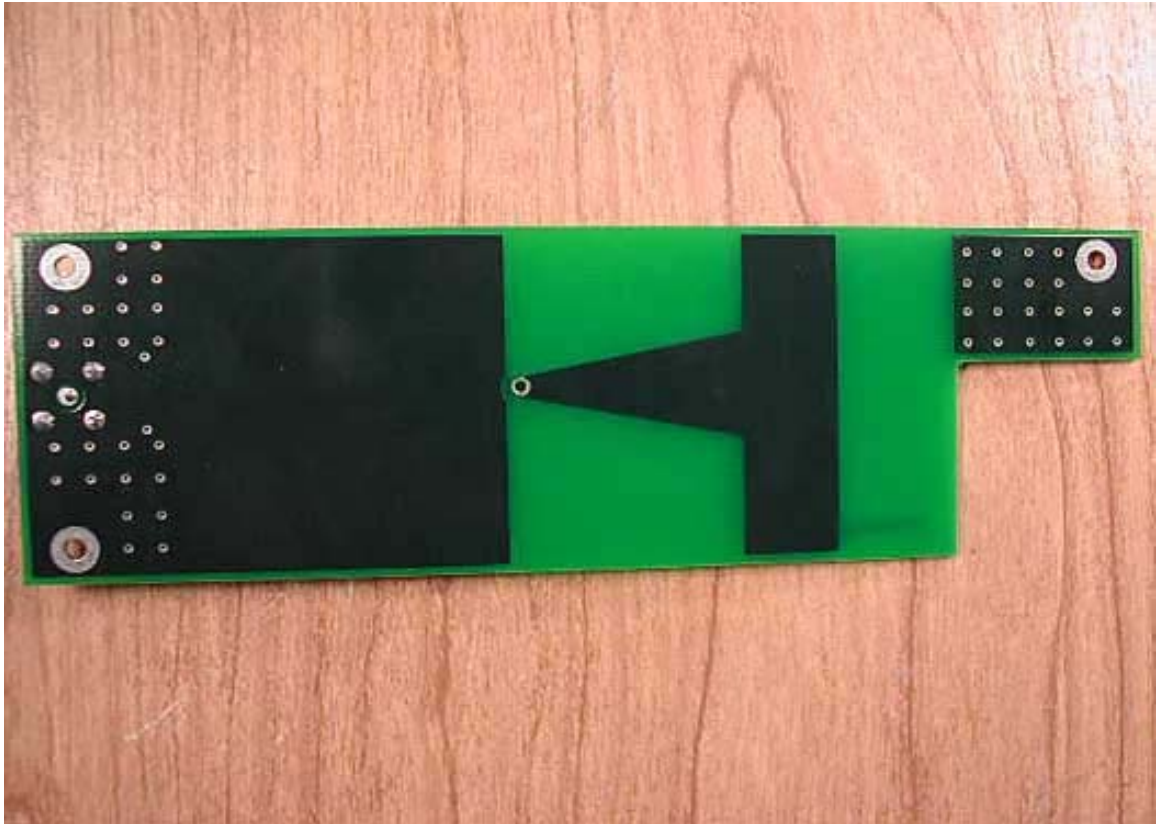
Antenna Front
