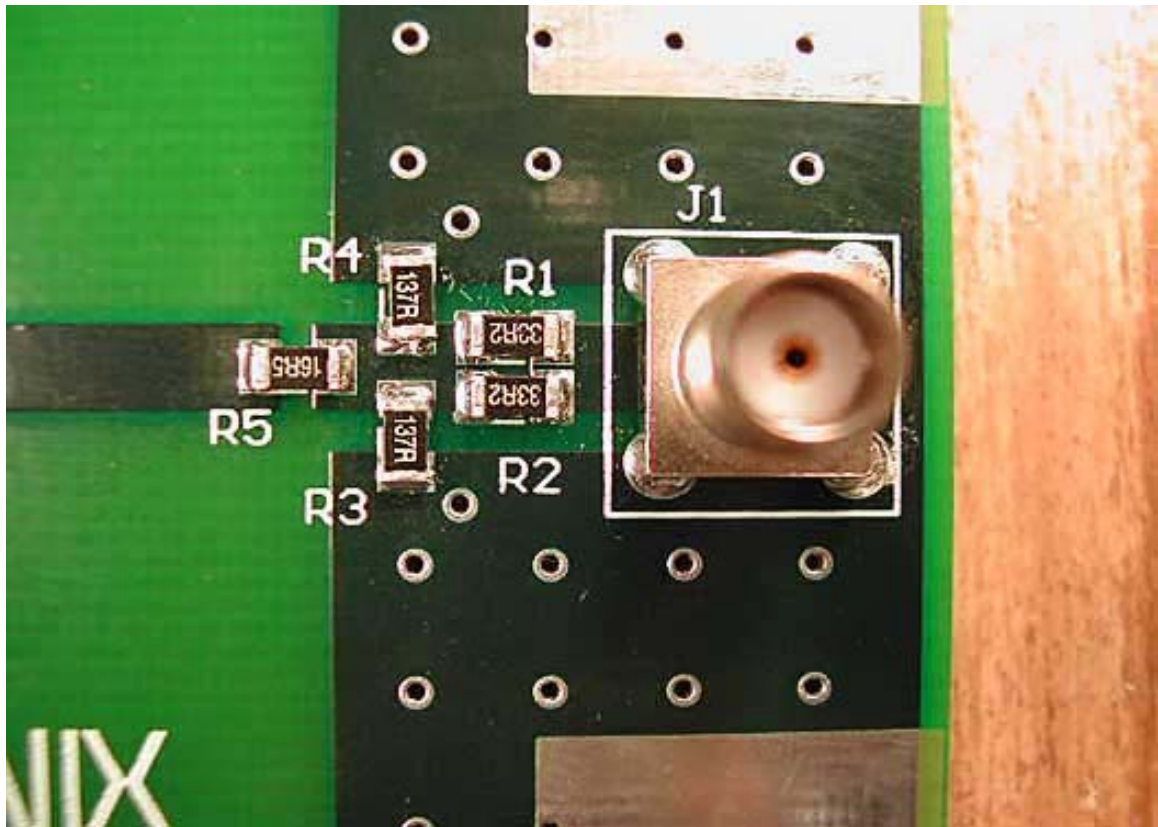
Antenna Close
