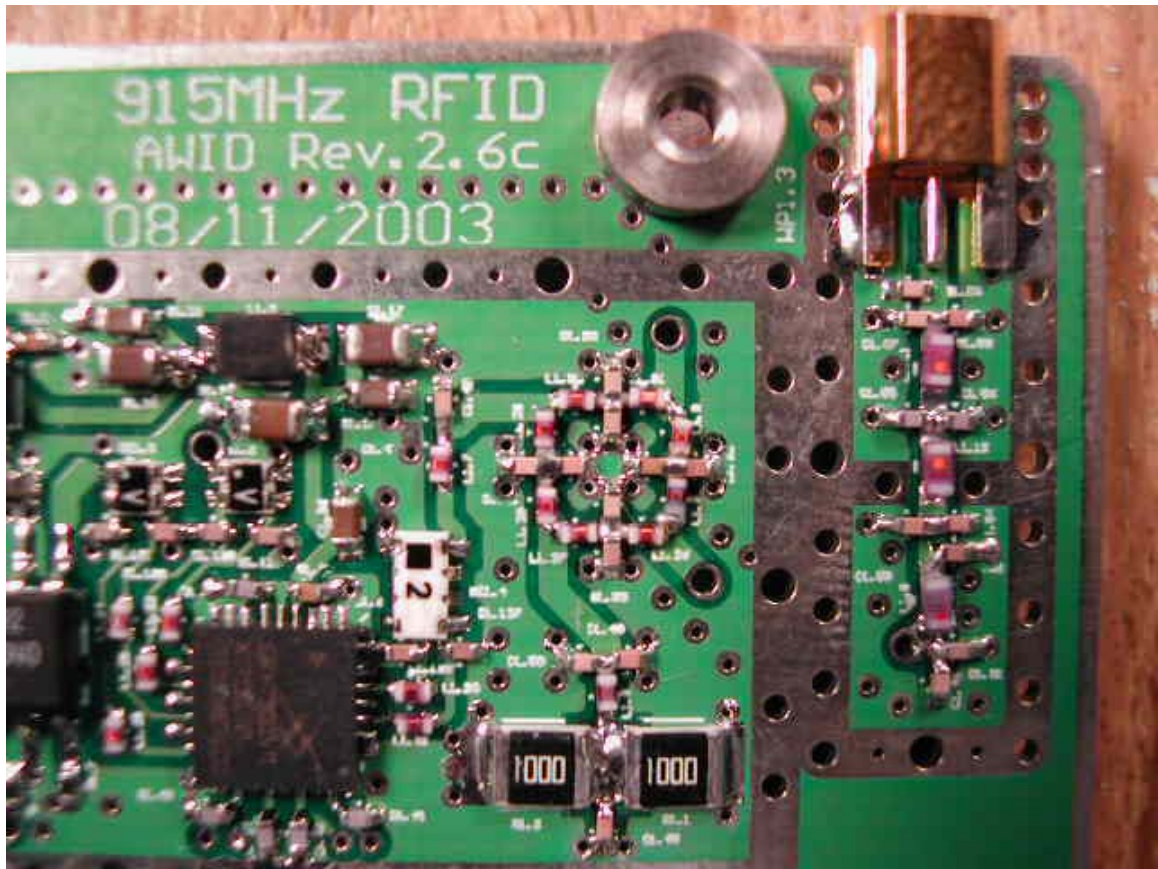
PCB Front 13
