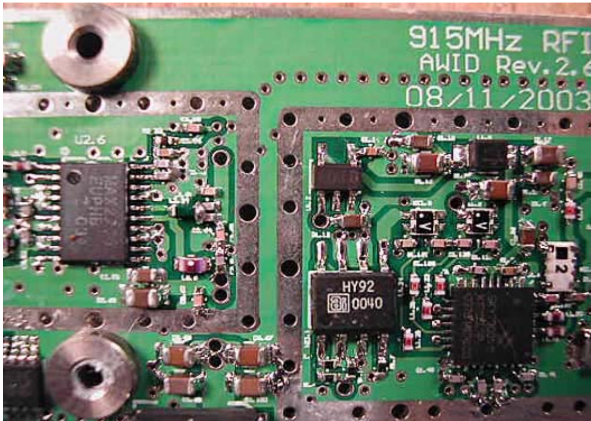
PCB Front 8
