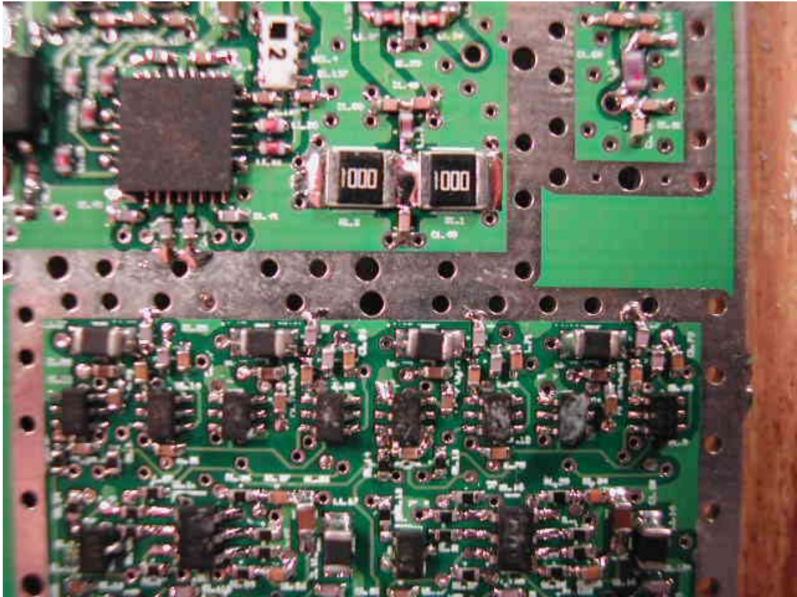
PCB Front 12
