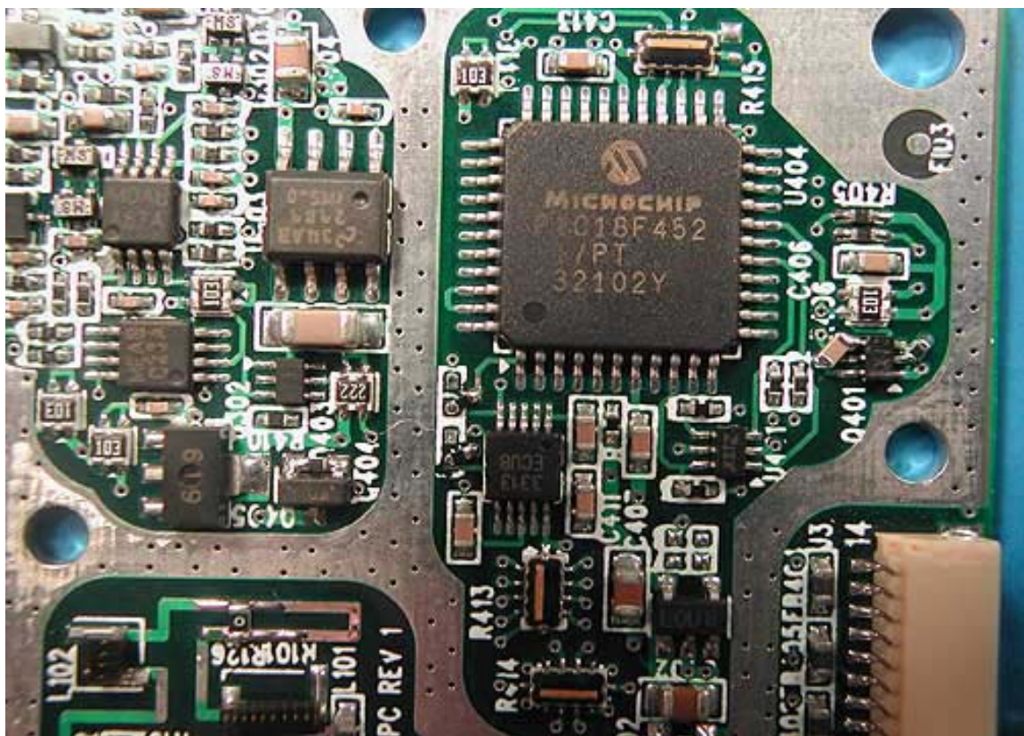
TX PCB 2
