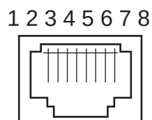
Figure 18. LAN Port (RJ-11) Pinout (Viewed from the outside of the radio.)
