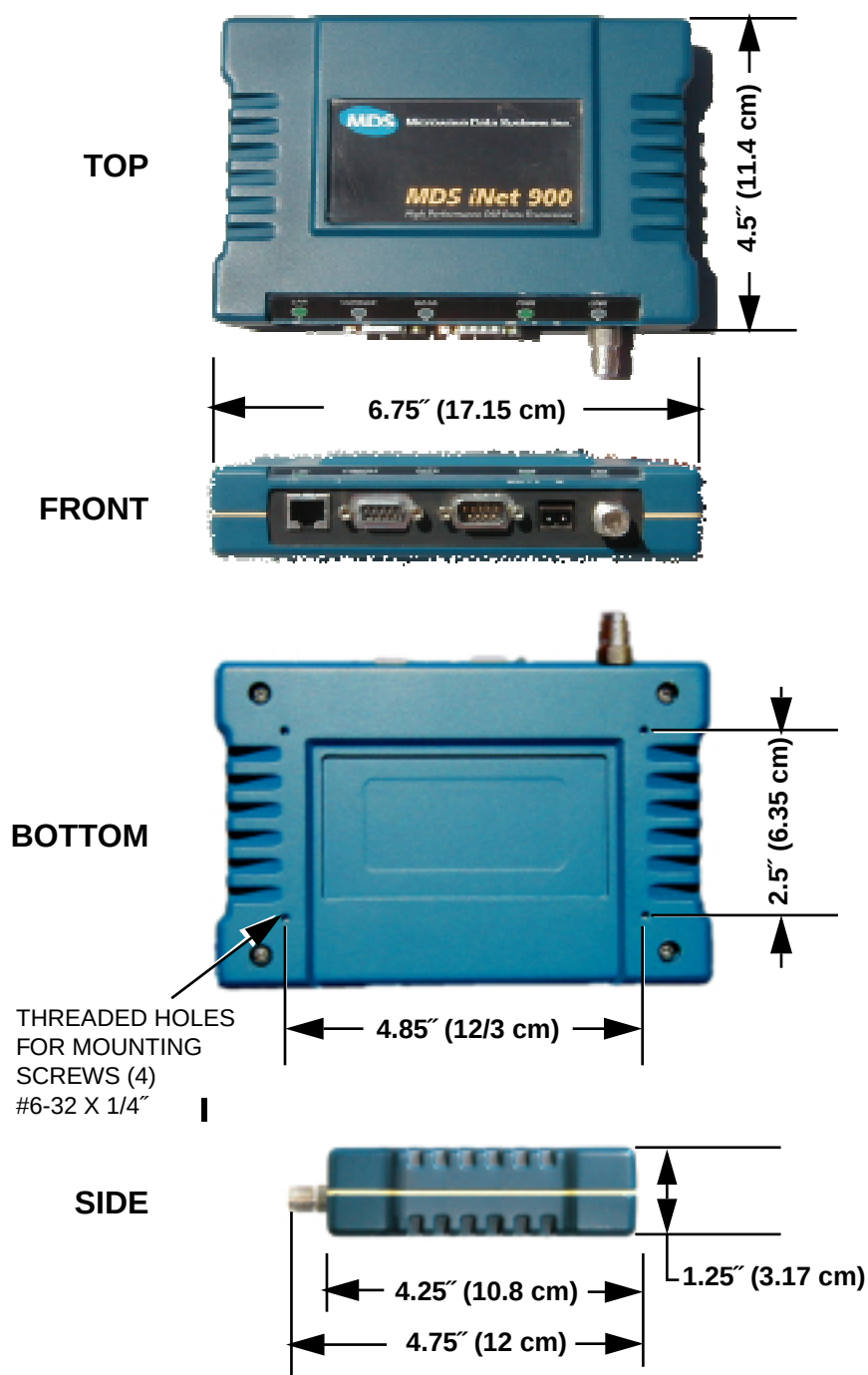
Figure 8. Transceiver dimensions
