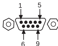
Figure 20. COM2 Port Viewed from the outside of the radio
