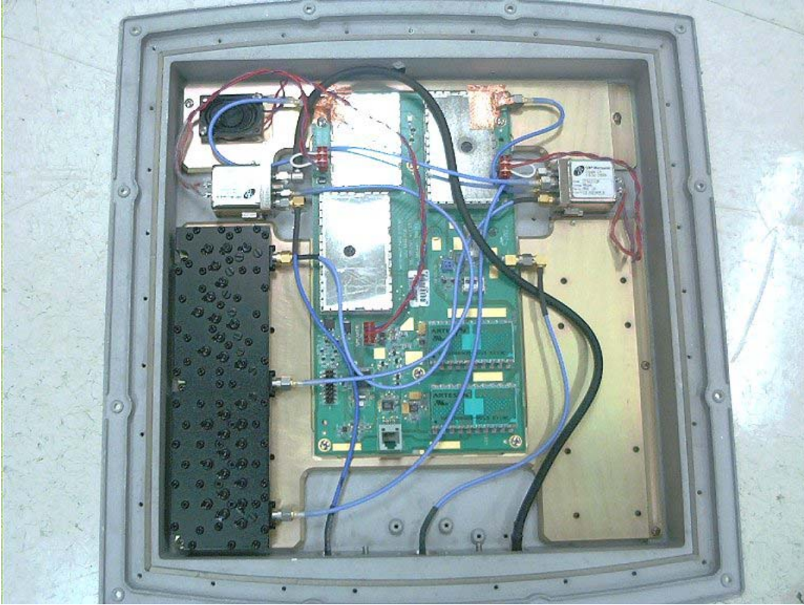
Duplexer location in the ODU
