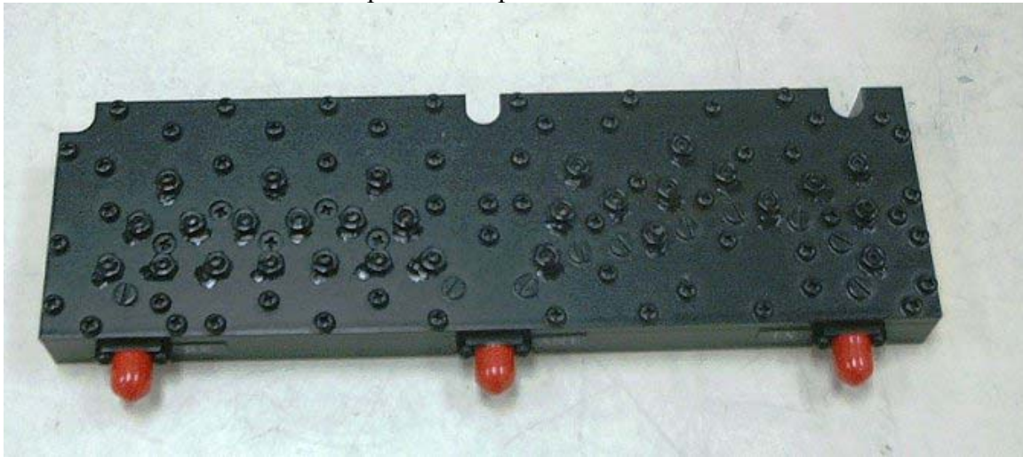
Duplexer – Top and Side Views
