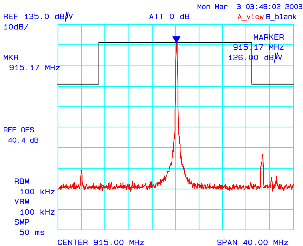
Plot 41: Radiated Emissions @ 3 Meters EUT with MDS ClearWave Omni-directional Base Station Antenna Channel: Mid, Tx. Frequency: 915 MHz, Modulation: 2 Level CPFSK Vertical Polarization
