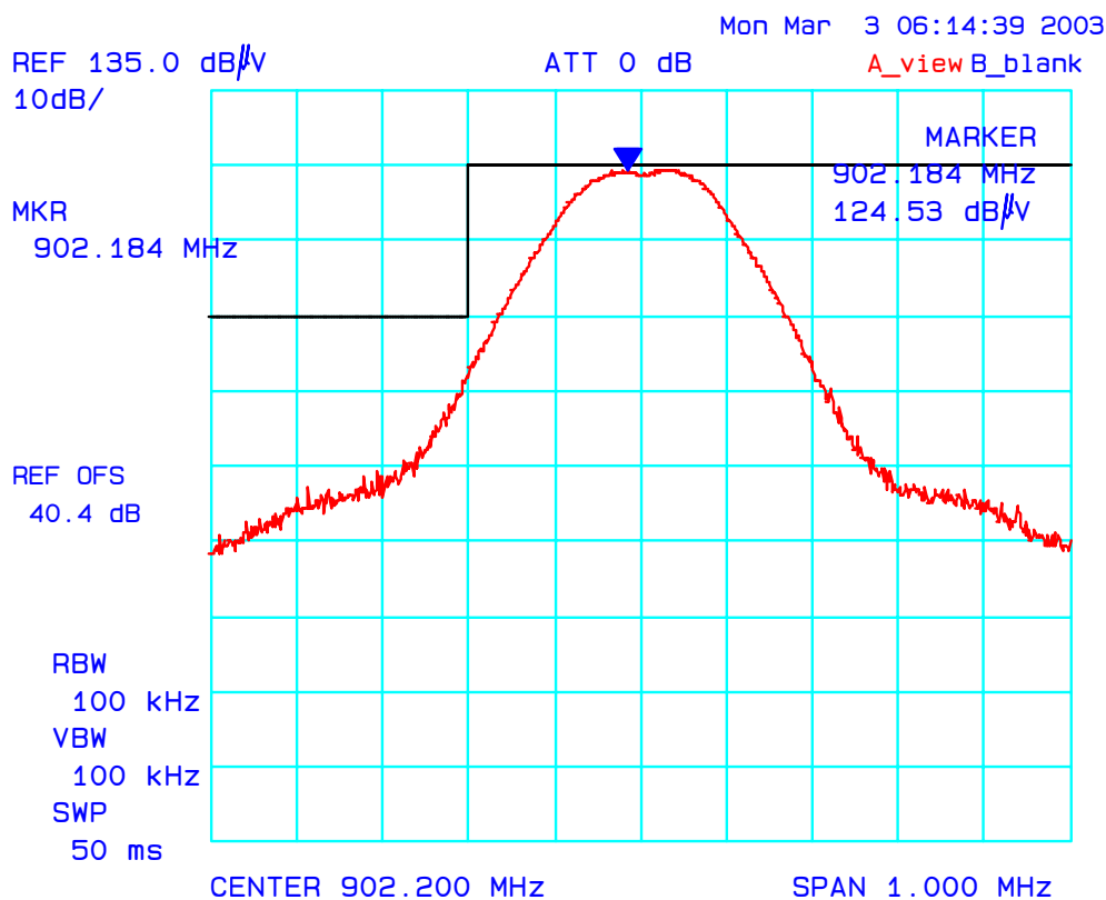
Plot 34: Radiated Emissions @ 3 Meters EUT with MDS ClearWave ½ Wave Dipole Antenna Channel: Low, Tx. Frequency: 902.2 MHz, Modulation: 2 Level CPFSK Horizontal Polarization
