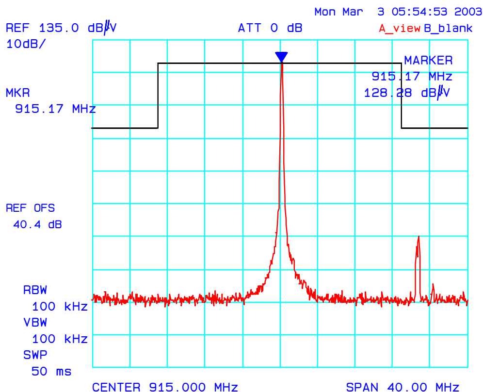
Plot 36: Radiated Emissions @ 3 Meters EUT with MDS ClearWave ½ Wave Dipole Antenna Channel: Mid, Tx. Frequency: 915 MHz, Modulation: 2 Level CPFSK Horizontal Polarization
