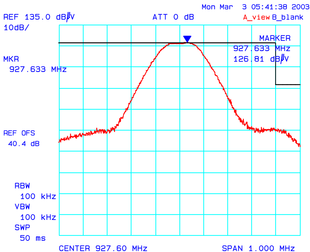
Plot 38: Radiated Emissions @ 3 Meters EUT with MDS ClearWave ½ Wave Dipole Antenna Channel: High, Tx. Frequency: 927.6 MHz, Modulation: 2 Level CPFSK Horizontal Polarization
