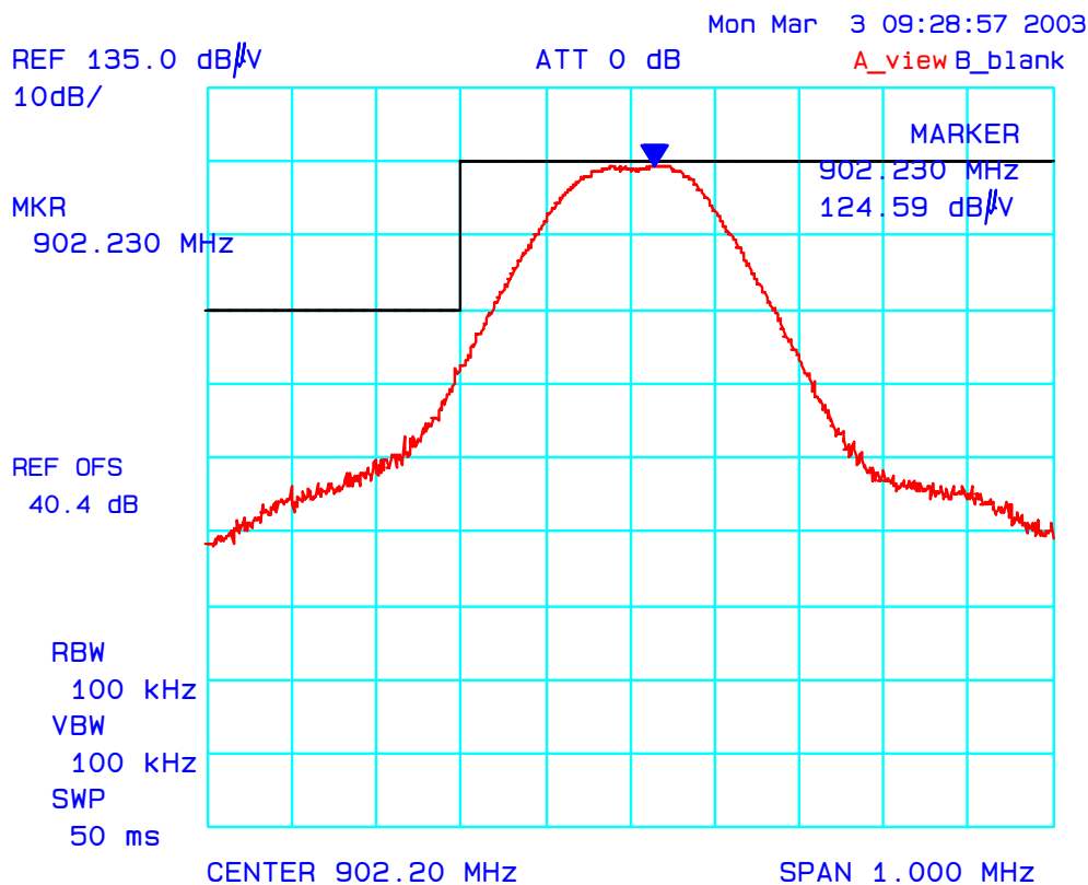
Plot 33: Radiated Emissions @ 3 Meters EUT with MDS ClearWave ½ Wave Dipole Antenna Channel: Low, Tx. Frequency: 902.2 MHz, Modulation: 2 Level CPFSK Vertical Polarization
