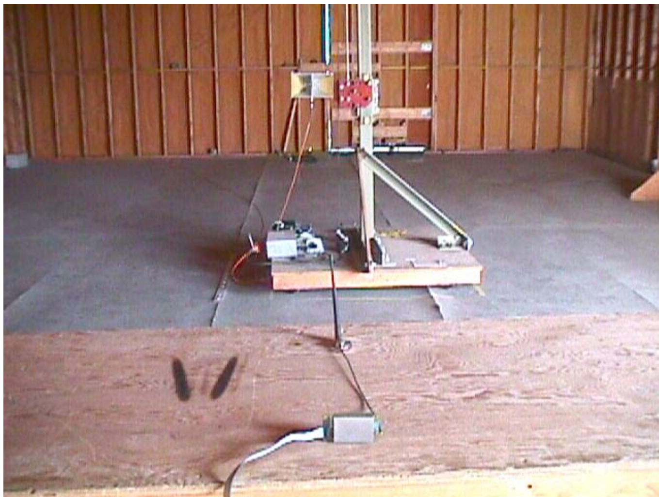
EUT with MDS ClearWave ½ Wave Dipole Antenna
