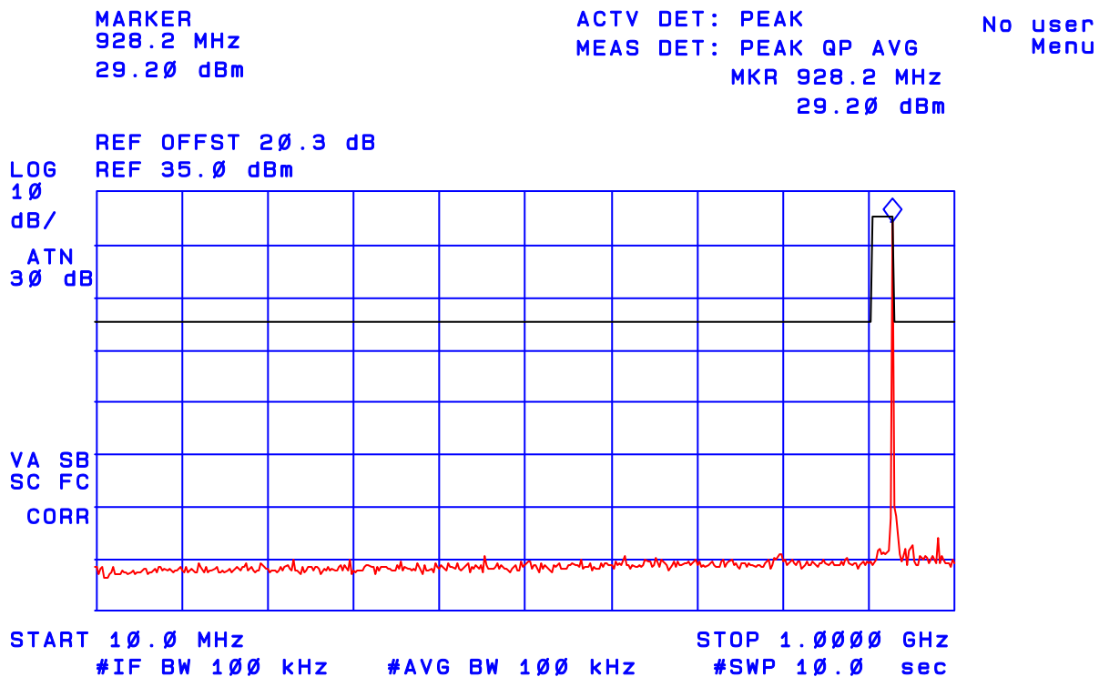
Plot 30: Spurious RF Conducted Emissions Channel: High, Tx. Frequency: 927.6 MHz, Modulation: 2 Level CPFSK
