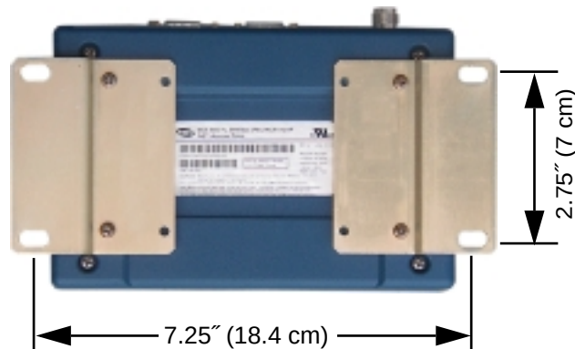
Figure 5-3. Mounting Brackets Dimensions
