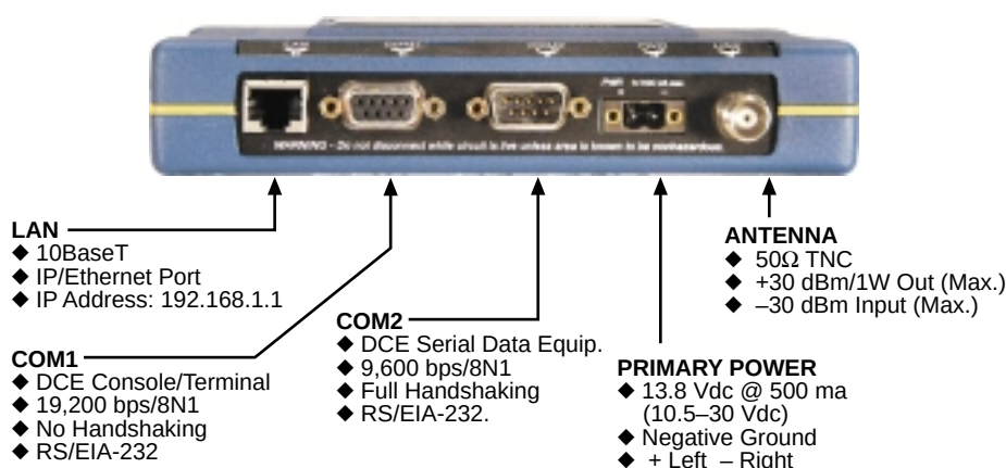
Figure 3-3. Transceiver (AP) Interface Default Configuration & Functions
