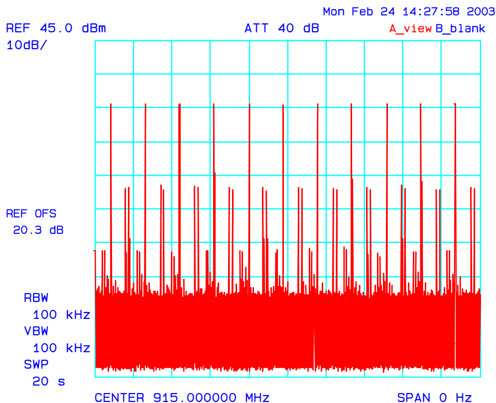
Plot 11: Average Time of Occupancy 28 ms Hop Dwell Setting Channel: Mid, Tx. Frequency: 915 MHz, Modulation: 2 Level CPFSK
