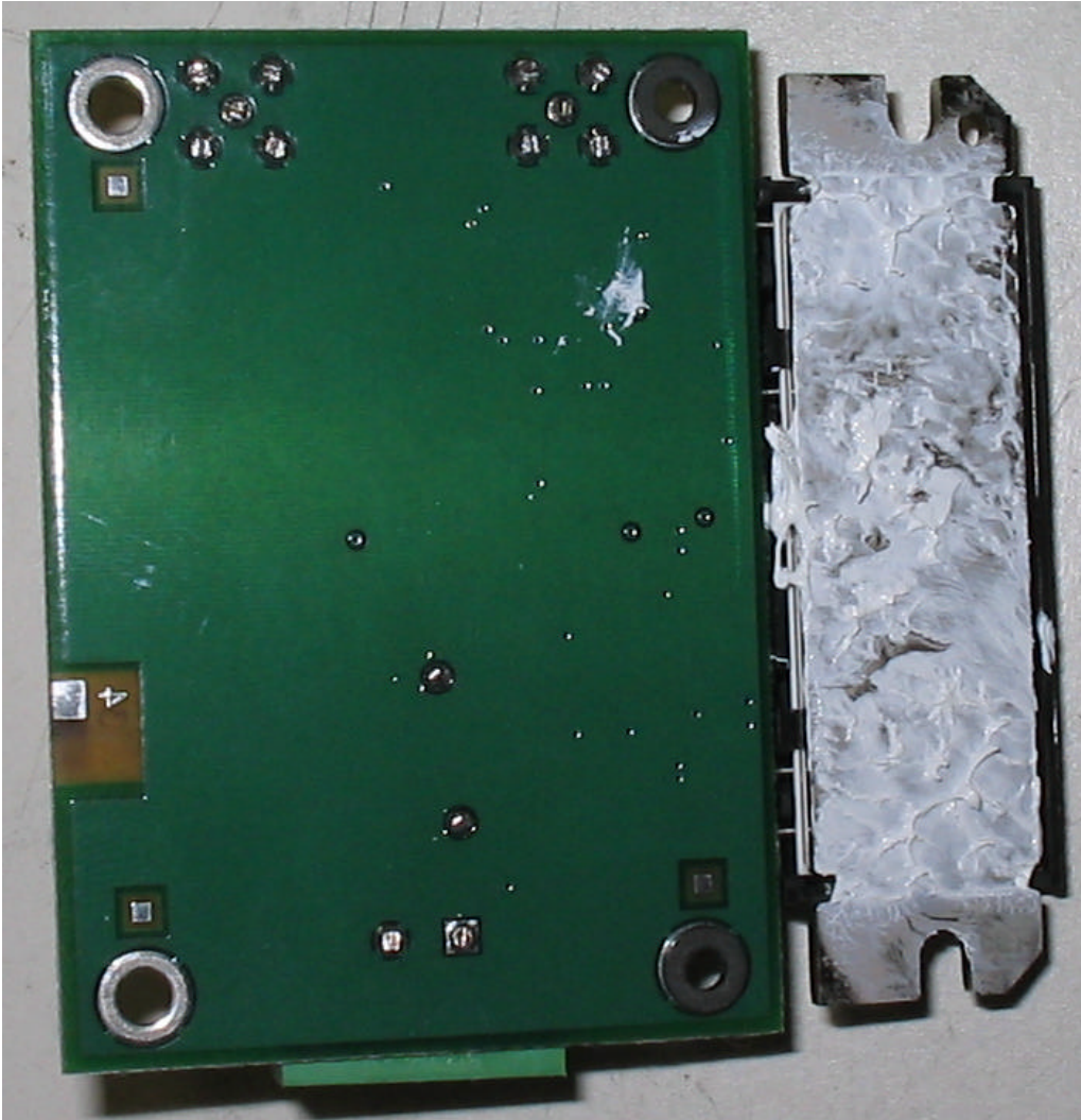
BACK SIDE OF AMPLIFIER BOARD
