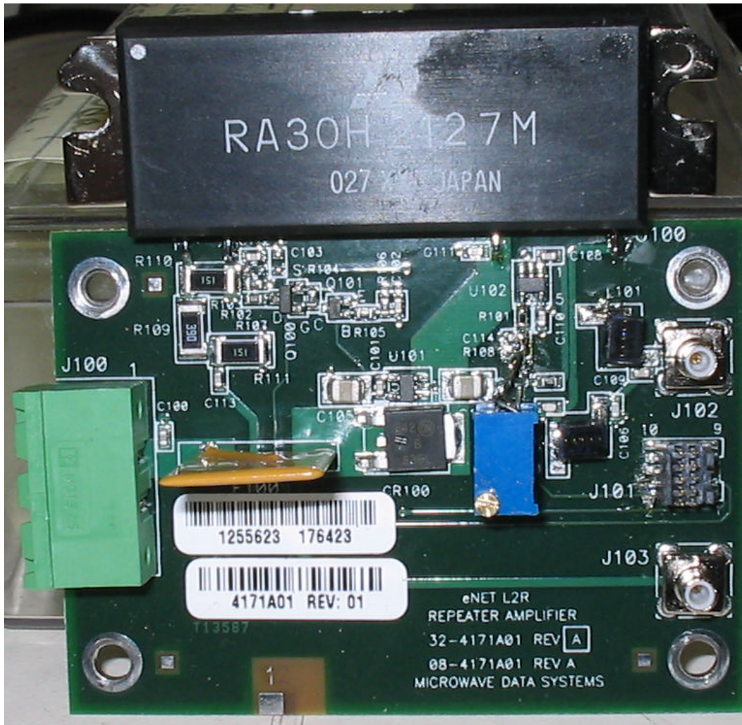
FRONT SIDE OF AMPLIFIER BOARD
