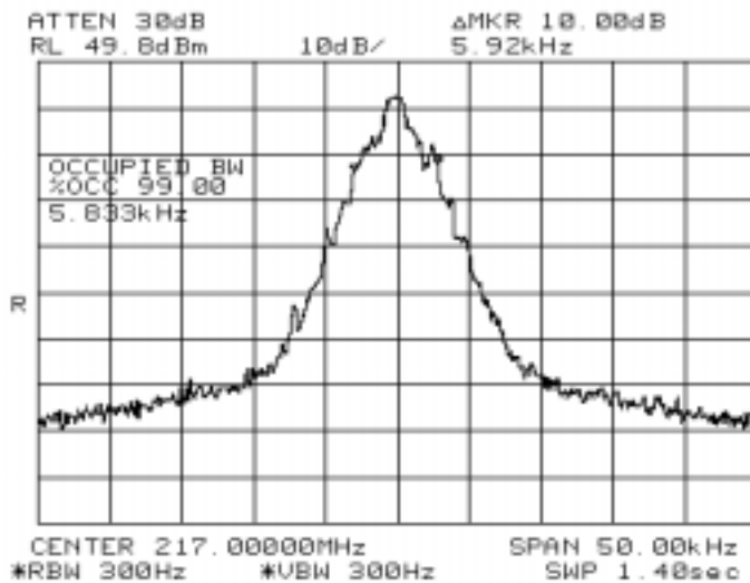
Amplifier Output Plot (217 MHz)
