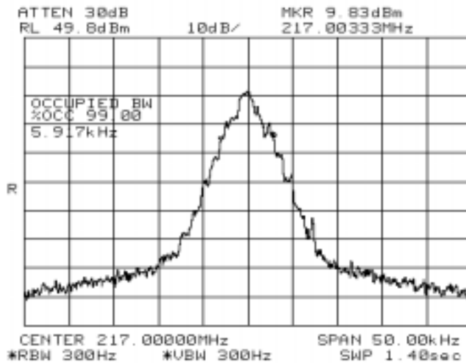
Input Plot (217MHz)
