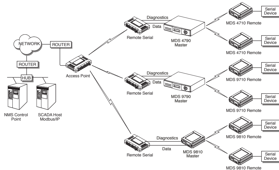
Figure 1-4. Backhaul Network
