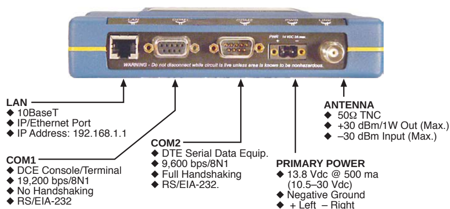
Figure 2-3. Interface Connectors, Functions & Defaults
