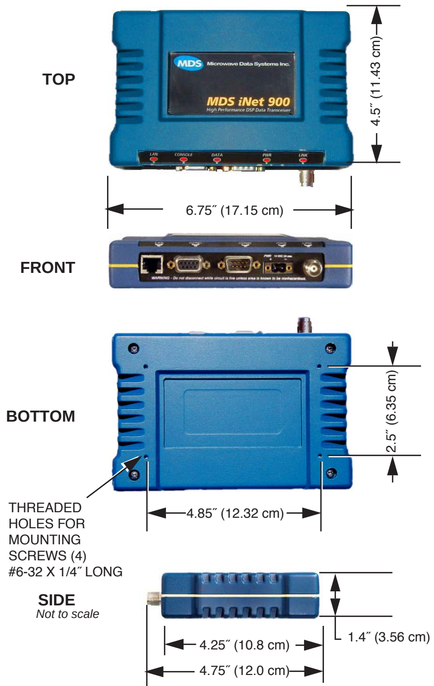
Figure 5-2. Transceiver Dimensions
