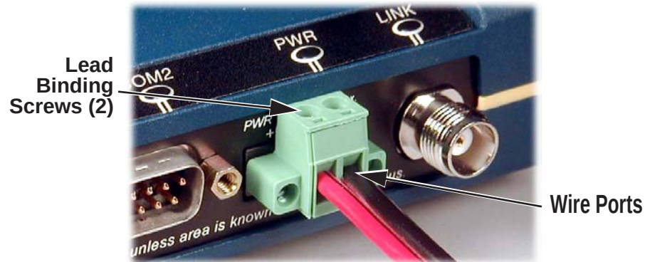
Figure 2-2. Power Connector, Polarity: Left +, Right –
