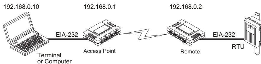
Figure 3-32. Point-to-Point Serial-to-Serial Application Diagram
