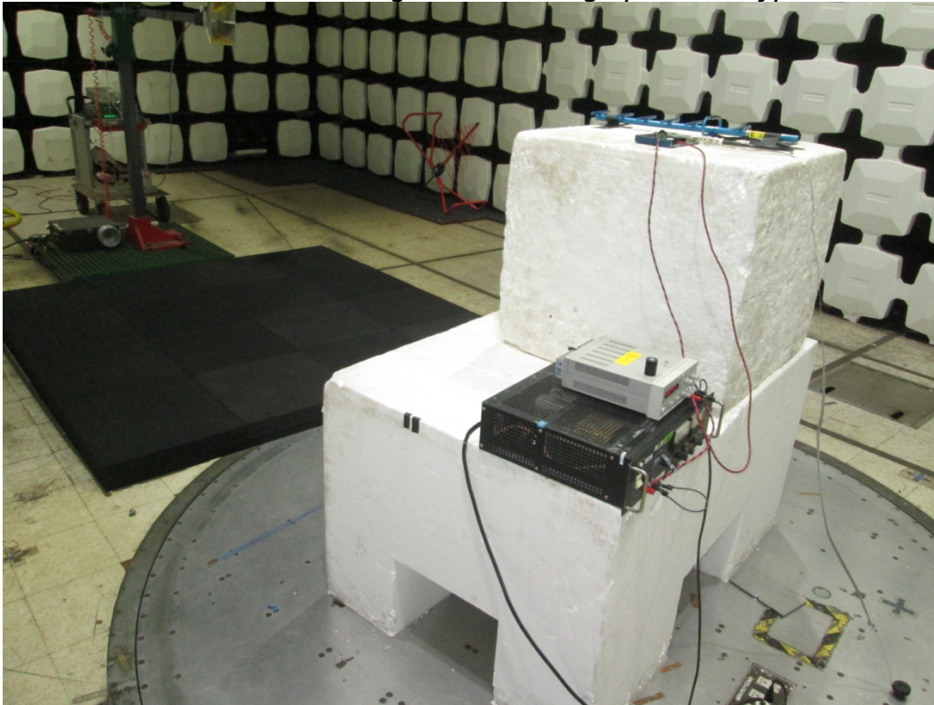
Radiated Emissions Test Configuration Photographs with Typical Antennas
