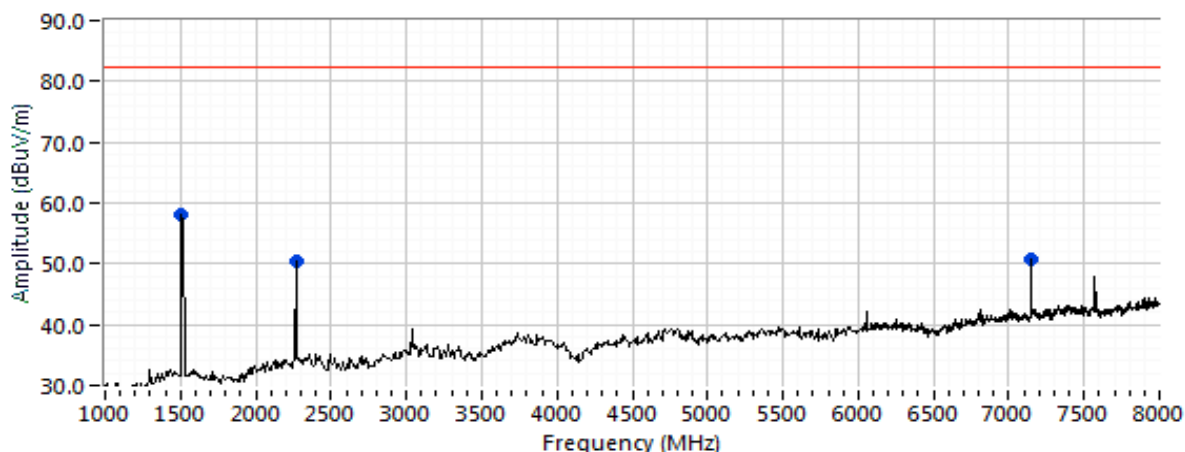
EUT at 757.5 MHz with antenna port terminated
