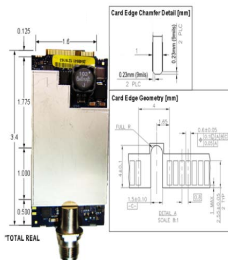
Figure 1. LW700 Transceiver Module (Mini PCI-Express Card Edge for Data/Power/& I/O and J700 Antenna)
