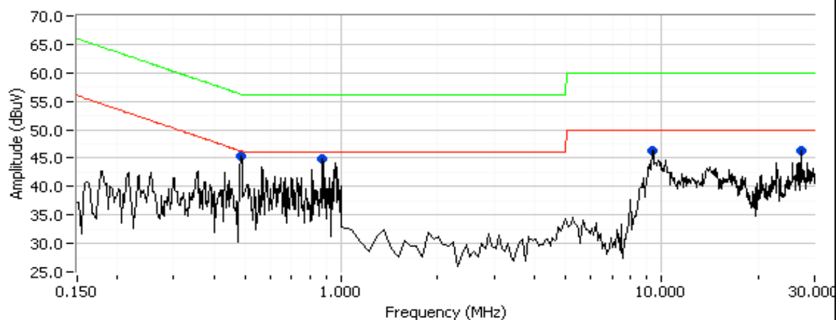
Run #1: .15-30MHz, Neutral
