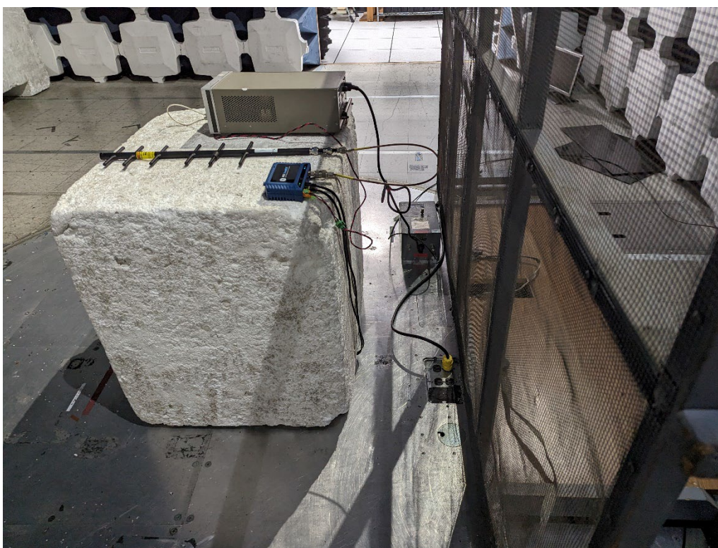
Conducted Emissions 2
