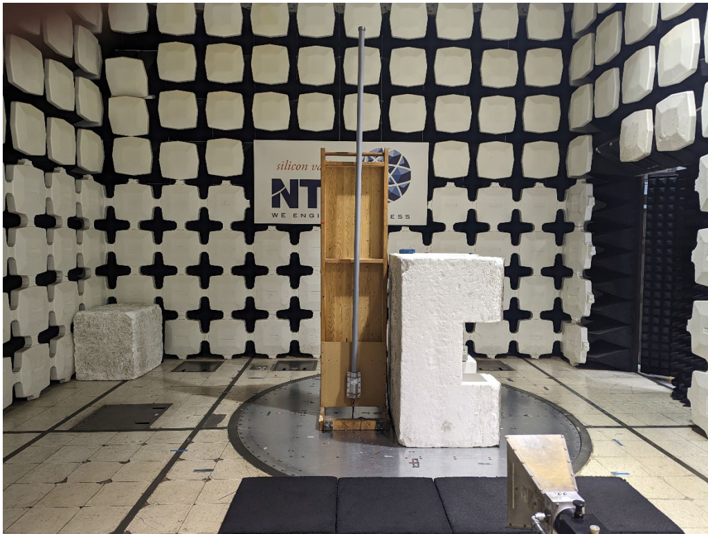
Above 1 GHz Tx Omni
