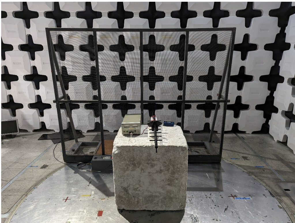
Conducted Emissions 1
