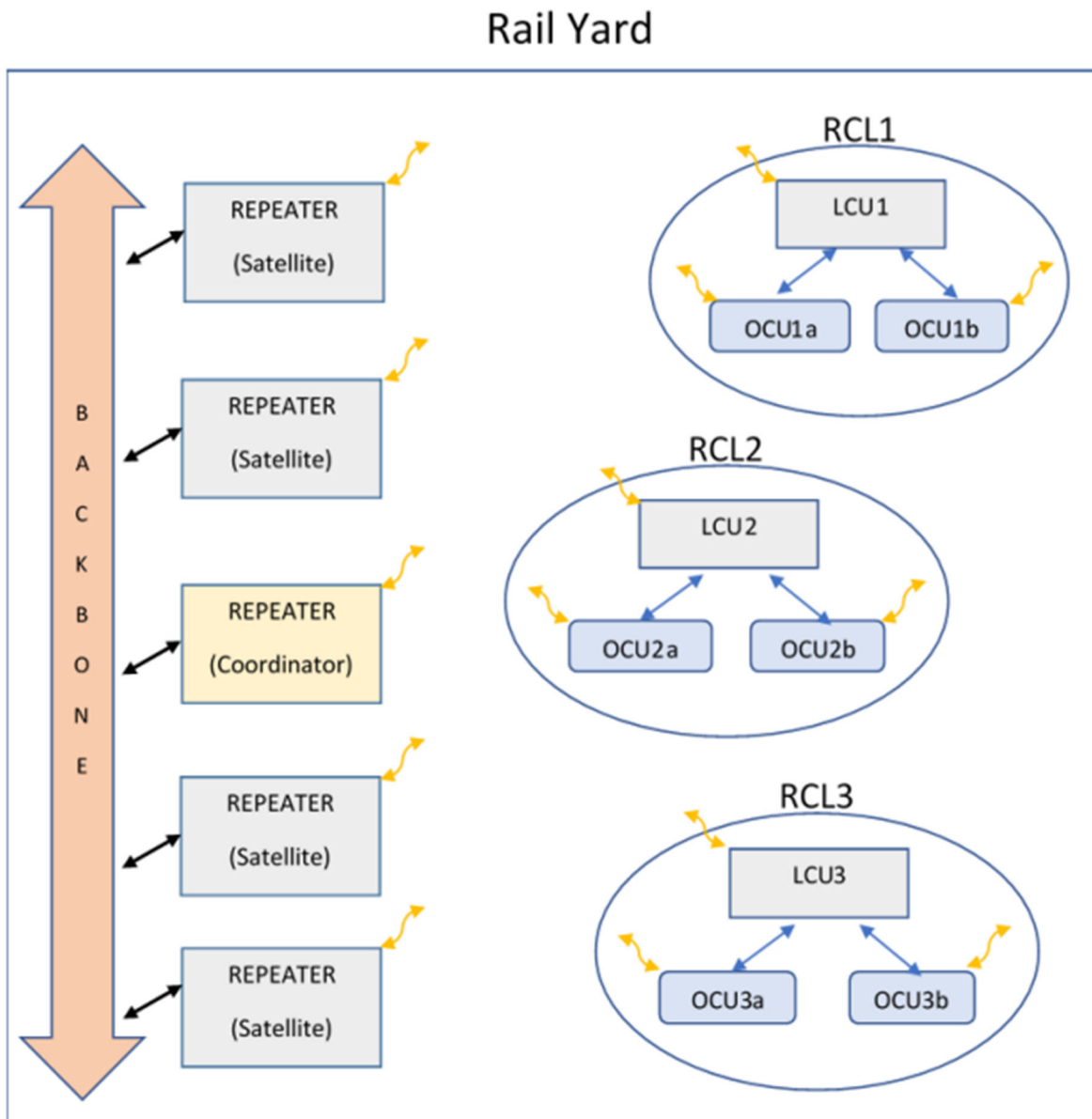
Figure 6: Multiple LCU-OCU Mode with Multiple Repeaters
