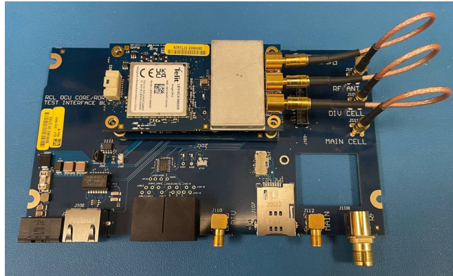
Figure 8: OCR220 Module Installed on test fixture
