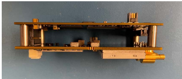
Figure 1: OCR220 Module. Bottom PCB is radio (Figure 2) and Top PCB is processor (Figure 3)
