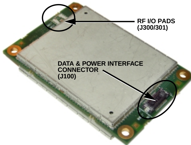
Figure 5. External Connections to the Transceiver Board (Bottom View of PCB)
