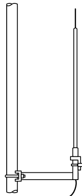
Figure 7. Typical Omni-directional Antenna for Master Stations (Shown mounted to mast)
