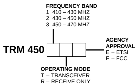
Figure 4. TRM 450 Model Number Codes (As found on the serial number and identification label)
