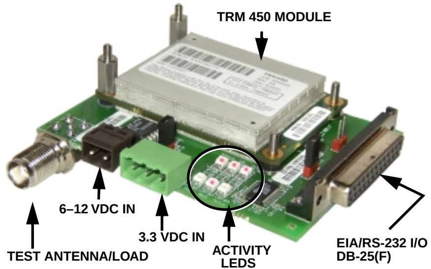
Figure 10. Test and Evaluation PCB Assembly (With TRM 450 module installed and retainers on RF connector end.)
