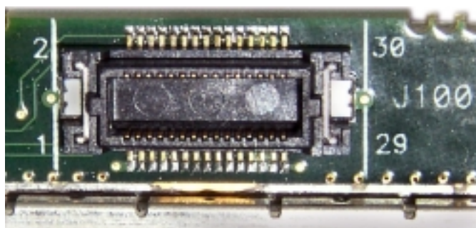
Figure 9. Data Interface Connector (As viewed from above)
