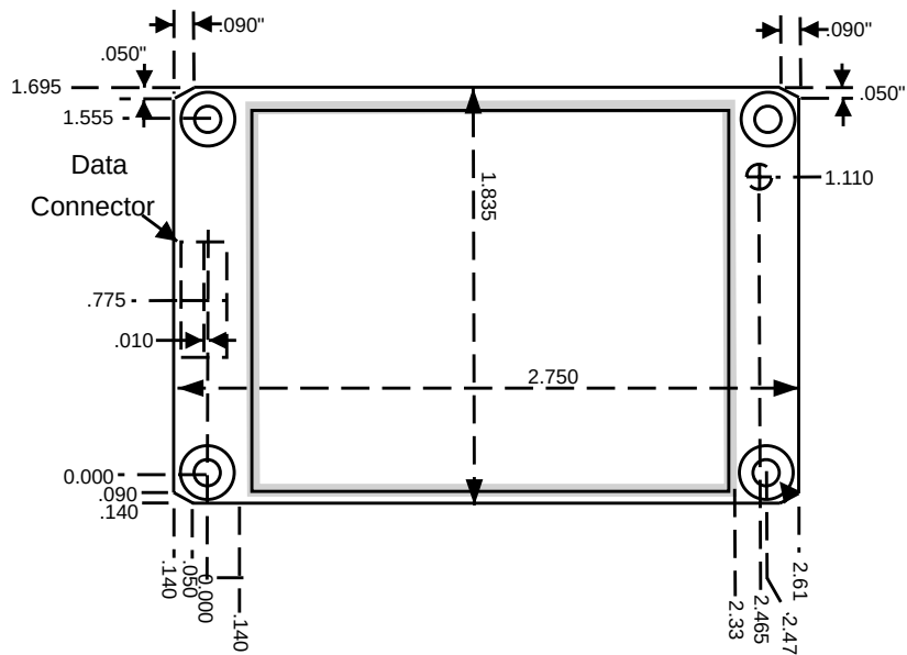
Figure 6. Transceiver Mounting Dimensions
