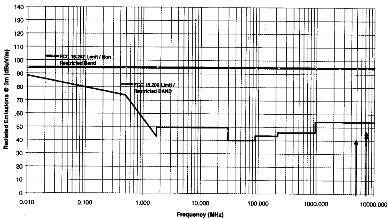
Transmitter Radiated Emissions Measurements at 3 Meter OETS Adaptive Broadband, MDS 24810 with SPG-36 External Antenna TRANSMIT Freq.: 2442.00 MHz
