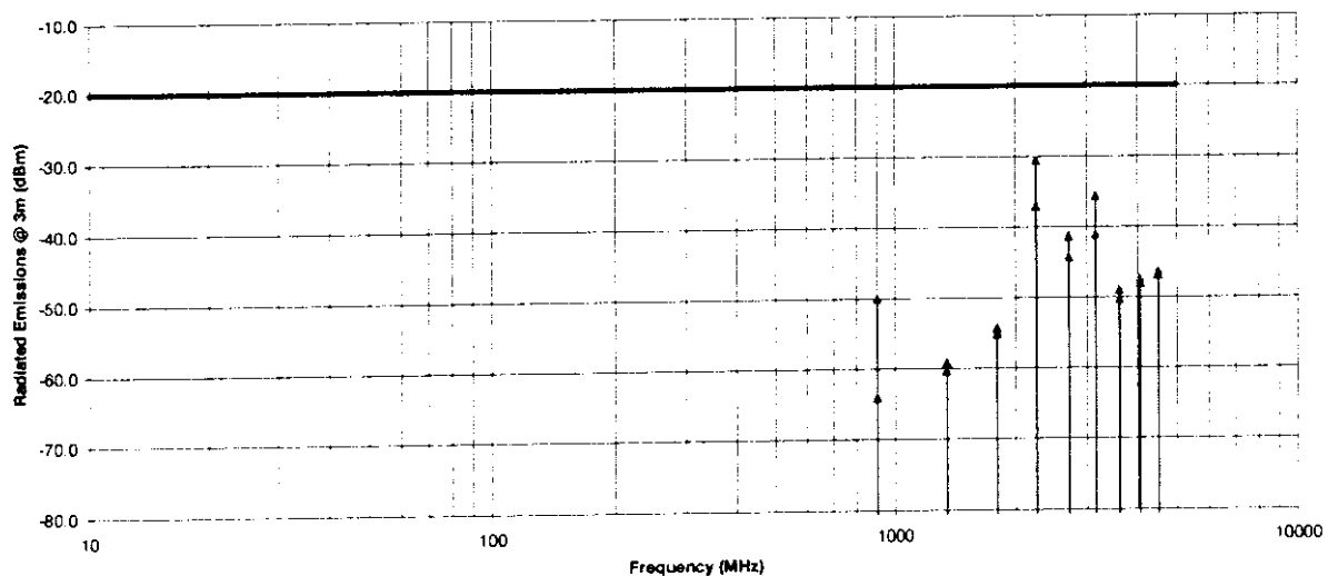
Transmitter Emissions Measurements at 3 Meter OFTS MICROWAVE DATA SYSTEMS - MDS 4790 UHF TRANSMITTER Center Frequency: 450 MHz, RF Output Power = 4.9 Watts Modulation: FM with internal random data source @ 9600 b/s
