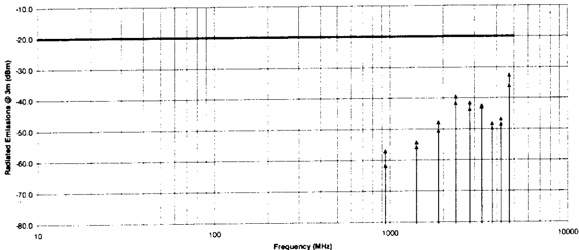
Transmitter Emissions Measurements at 3 Meter OETS MICROWAVE DATA SYSTEMS - MDS 4790 UHF TRANSMITTER Center Frequnc: 470 MHz, RF Ouput Power = 5.4 Watts Modulation: FM with internal random data source @ 9600 b/s
