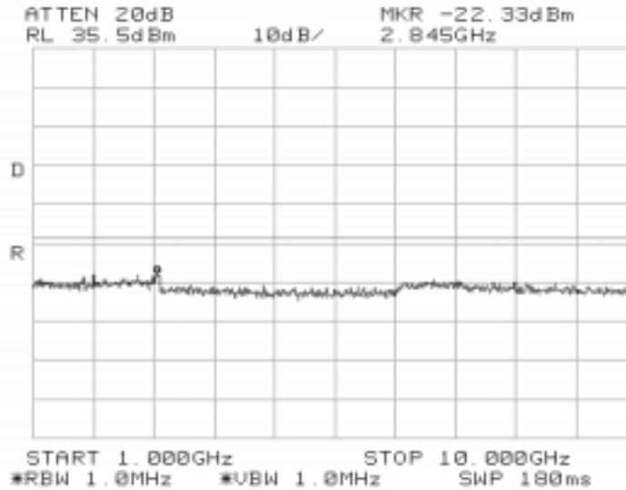
Graph T60106/502
