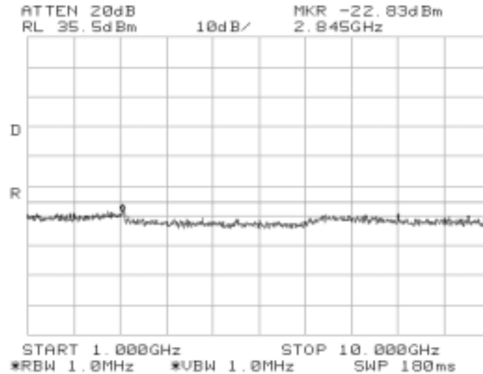
Graph T60106/506
