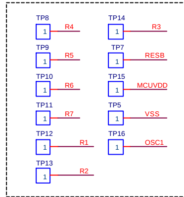
OTP TYPE BURN IN PIN
