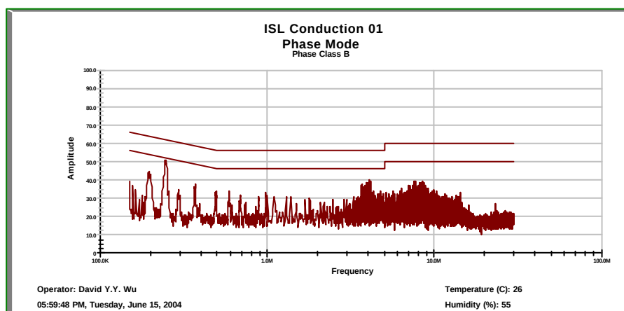
Graph 2.3.1 Power Line Conducted Emissions (Hot)
