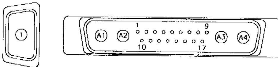
Figure 2-1. Amplifier Connectors (on Rear of MCA9129-90 Module)
