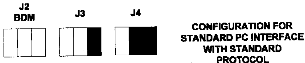
Figure 2-5. Jumper Settings
