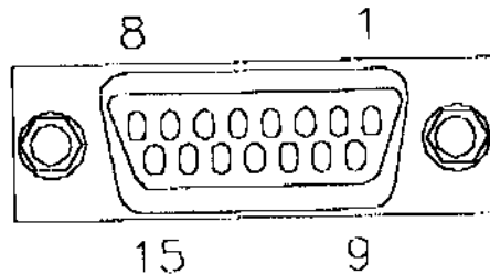
Figure 2-2. ALARMS Connector
